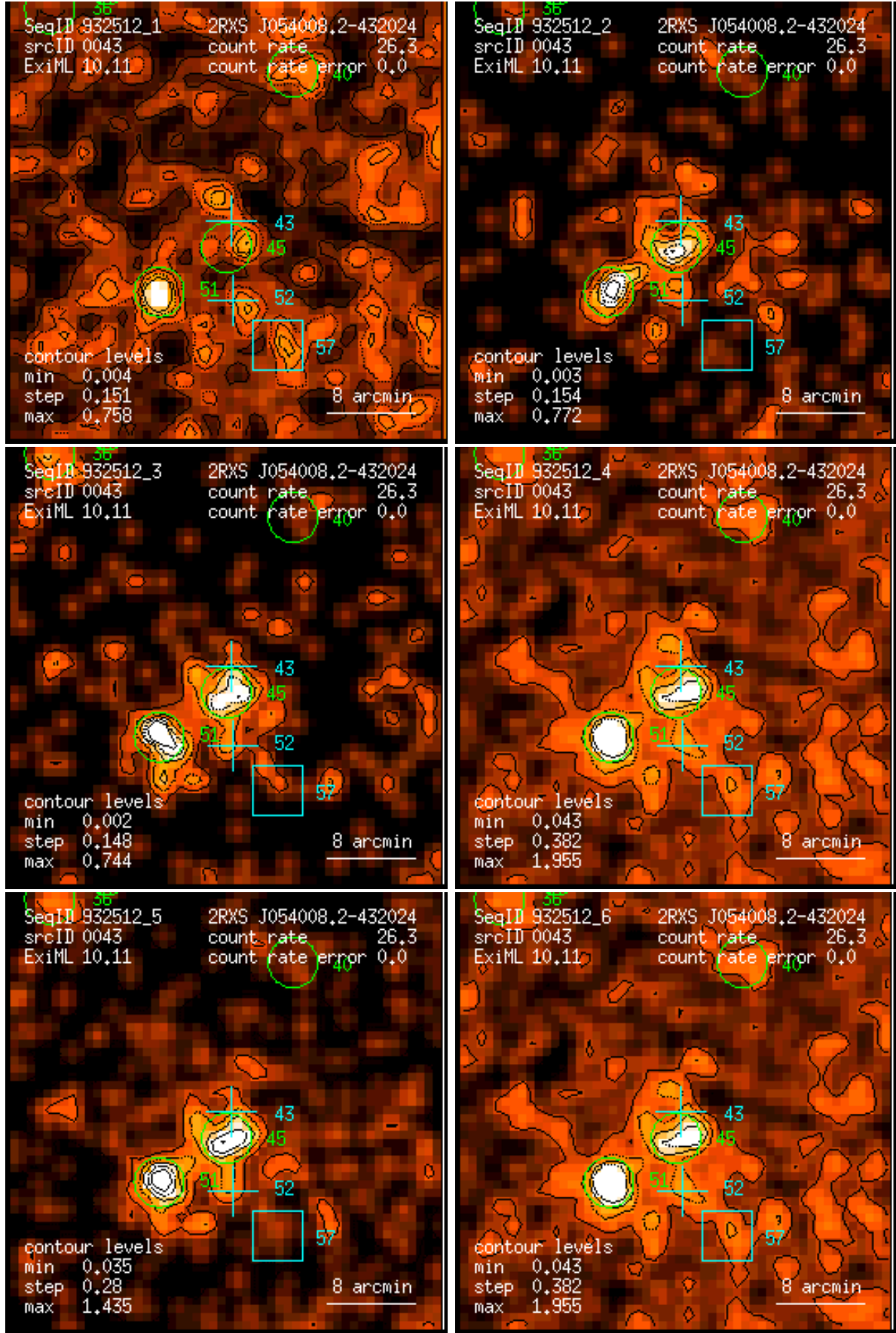
Figure 43: RASS 932512: detection 0043: band rate images, Gaussian filter: (1) PSPC channels 11 – 41, (2) 52 – 90, (3) 91 – 201, (4) 11 – 235, (5) 52 – 201, (6) 11 – 201. Broad band rates in counts/ks. Band rate contour levels in counts/ks/arcmin 2 .
