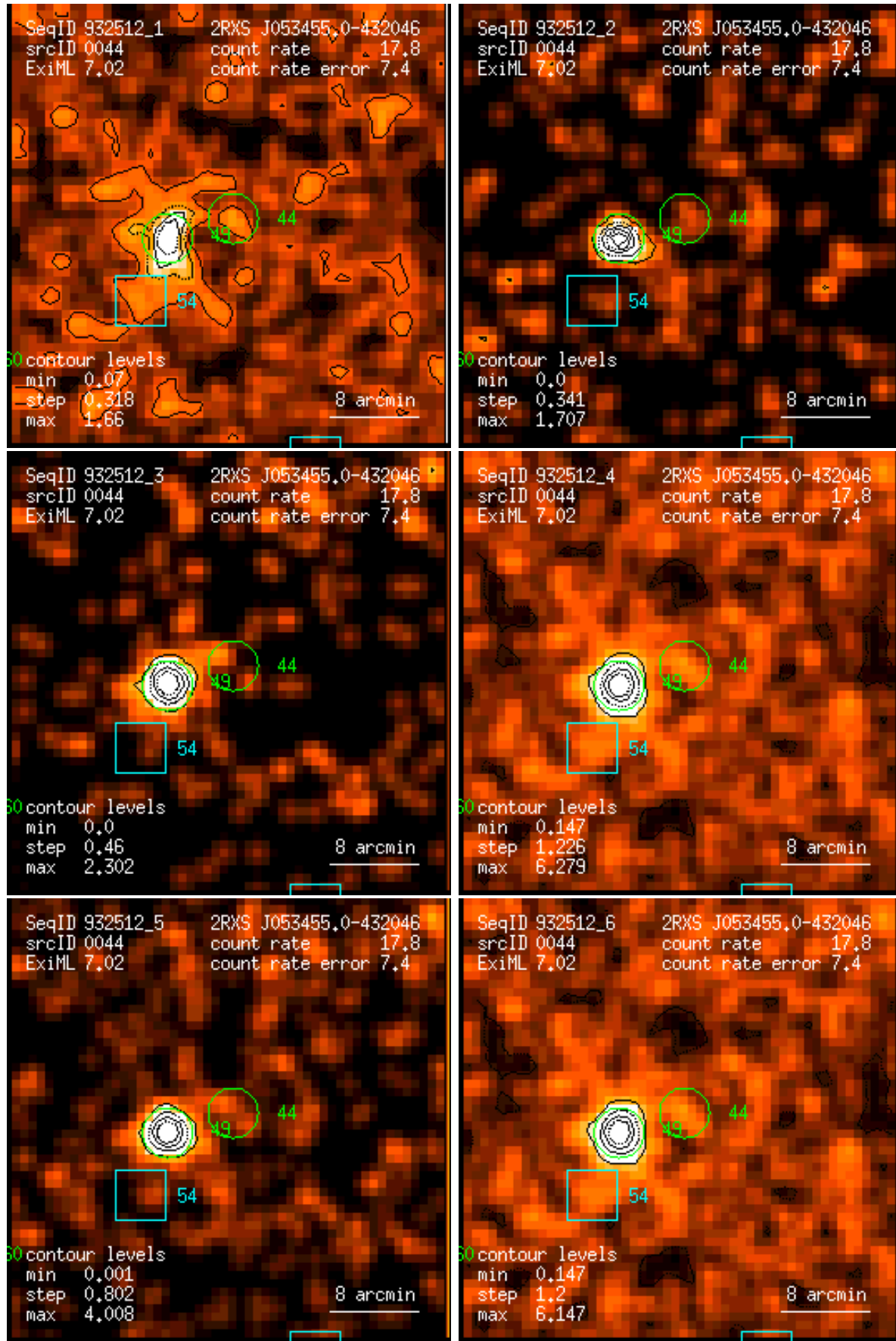
Figure 44: RASS 932512: detection 0044: band rate images, Gaussian filter: (1) PSPC channels 11 – 41, (2) 52 – 90, (3) 91 – 201, (4) 11 – 235, (5) 52 – 201, (6) 11 – 201. Broad band rates in counts/ks. Band rate contour levels in counts/ks/arcmin 2 .
