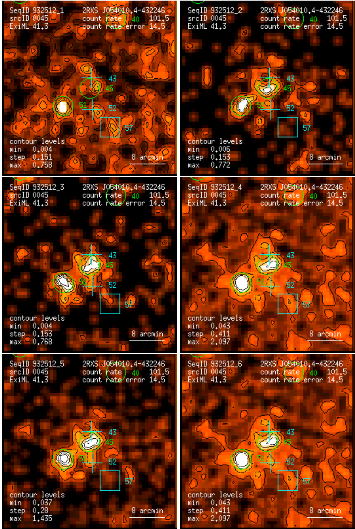
Figure 45: RASS 932512: detection 0045: band rate images, Gaussian filter: (1) PSPC channels 11 – 41, (2) 52 – 90, (3) 91 – 201, (4) 11 – 235, (5) 52 – 201, (6) 11 – 201. Broad band rates in counts/ks. Band rate contour levels in counts/ks/arcmin 2 .
