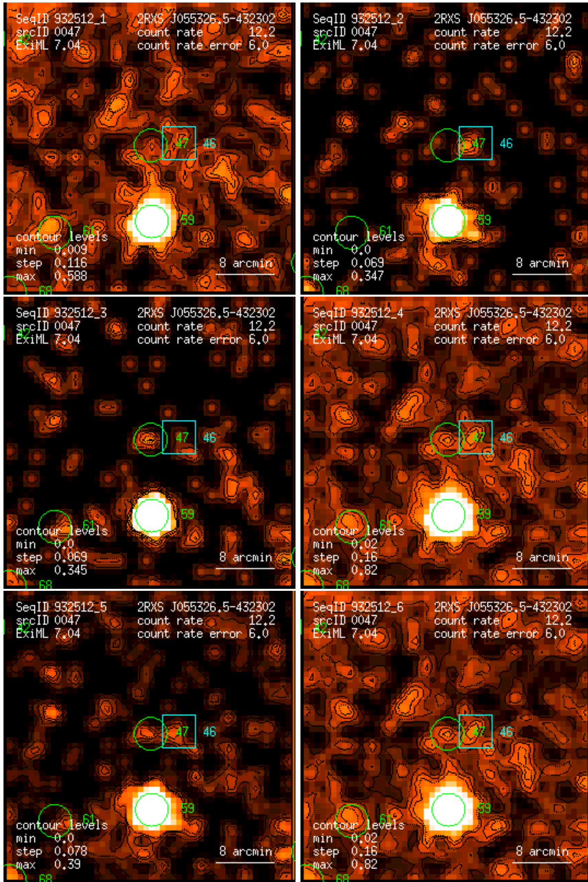
Figure 47: RASS 932512: detection 0047: band rate images, Gaussian filter: (1) PSPC channels 11 – 41, (2) 52 – 90, (3) 91 – 201, (4) 11 – 235, (5) 52 – 201, (6) 11 – 201. Broad band rates in counts/ks. Band rate contour levels in counts/ks/arcmin 2 .
