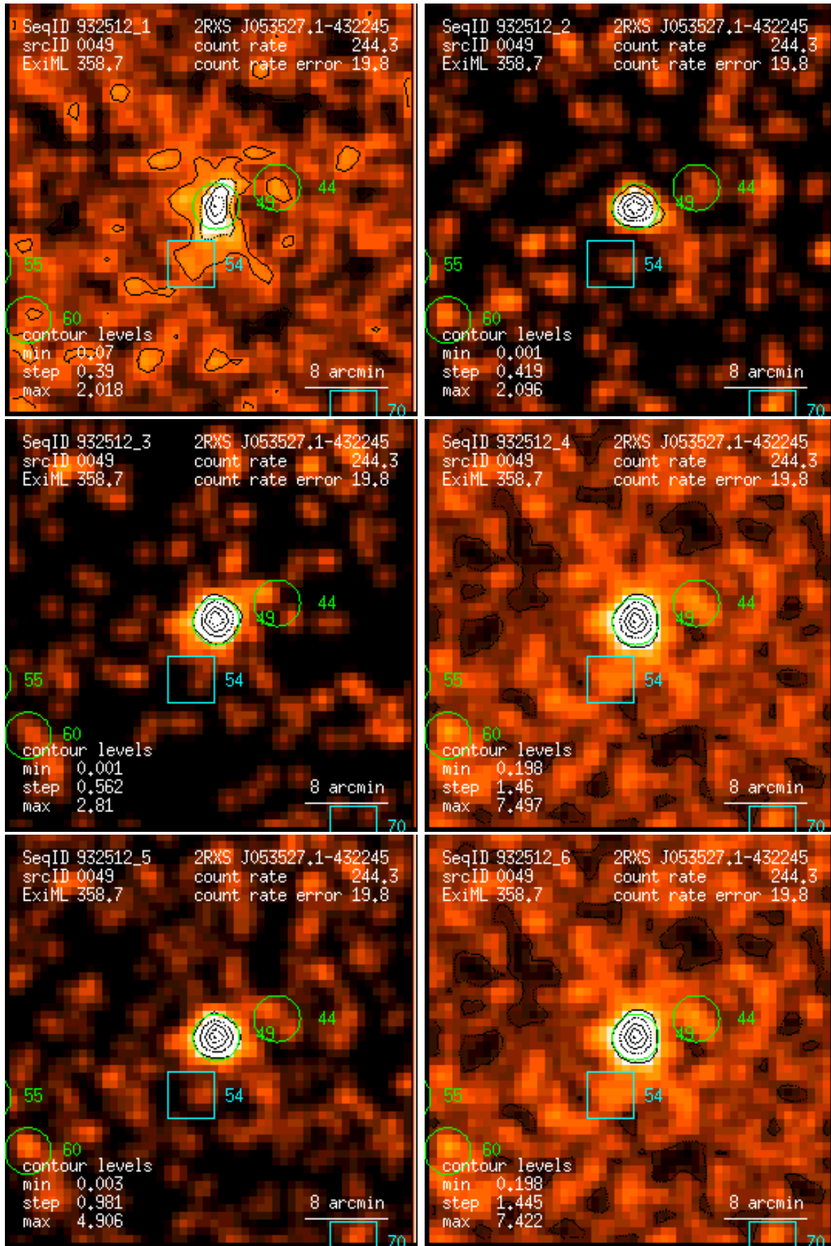
Figure 49: RASS 932512: detection 0049: band rate images, Gaussian filter: (1) PSPC channels 11 – 41, (2) 52 – 90, (3) 91 – 201, (4) 11 – 235, (5) 52 – 201, (6) 11 – 201. Broad band rates in counts/ks. Band rate contour levels in counts/ks/arcmin 2 .
