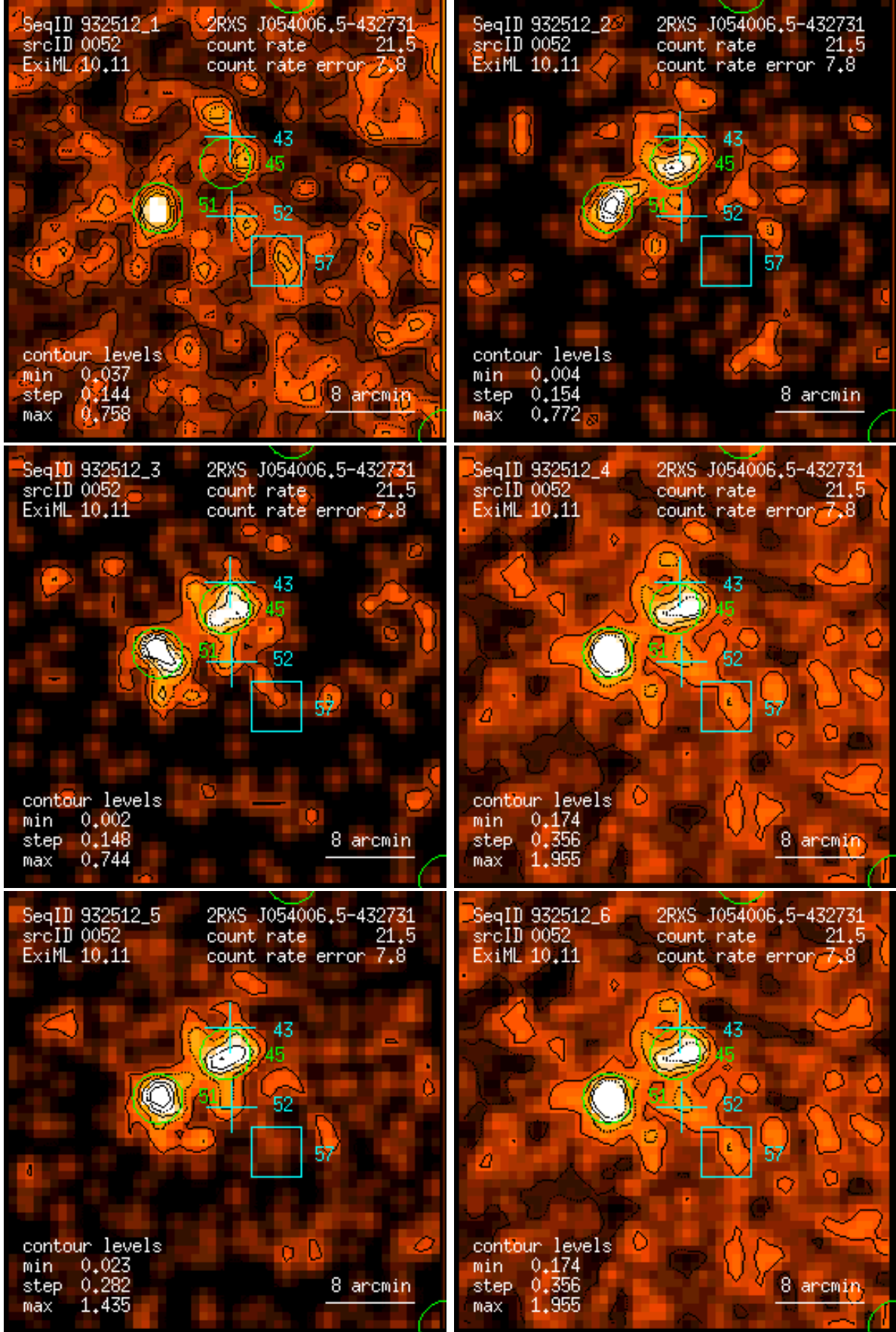
Figure 52: RASS 932512: detection 0052: band rate images, Gaussian filter: (1) PSPC channels 11 – 41, (2) 52 – 90, (3) 91 – 201, (4) 11 – 235, (5) 52 – 201, (6) 11 – 201. Broad band rates in counts/ks. Band rate contour levels in counts/ks/arcmin 2 .
