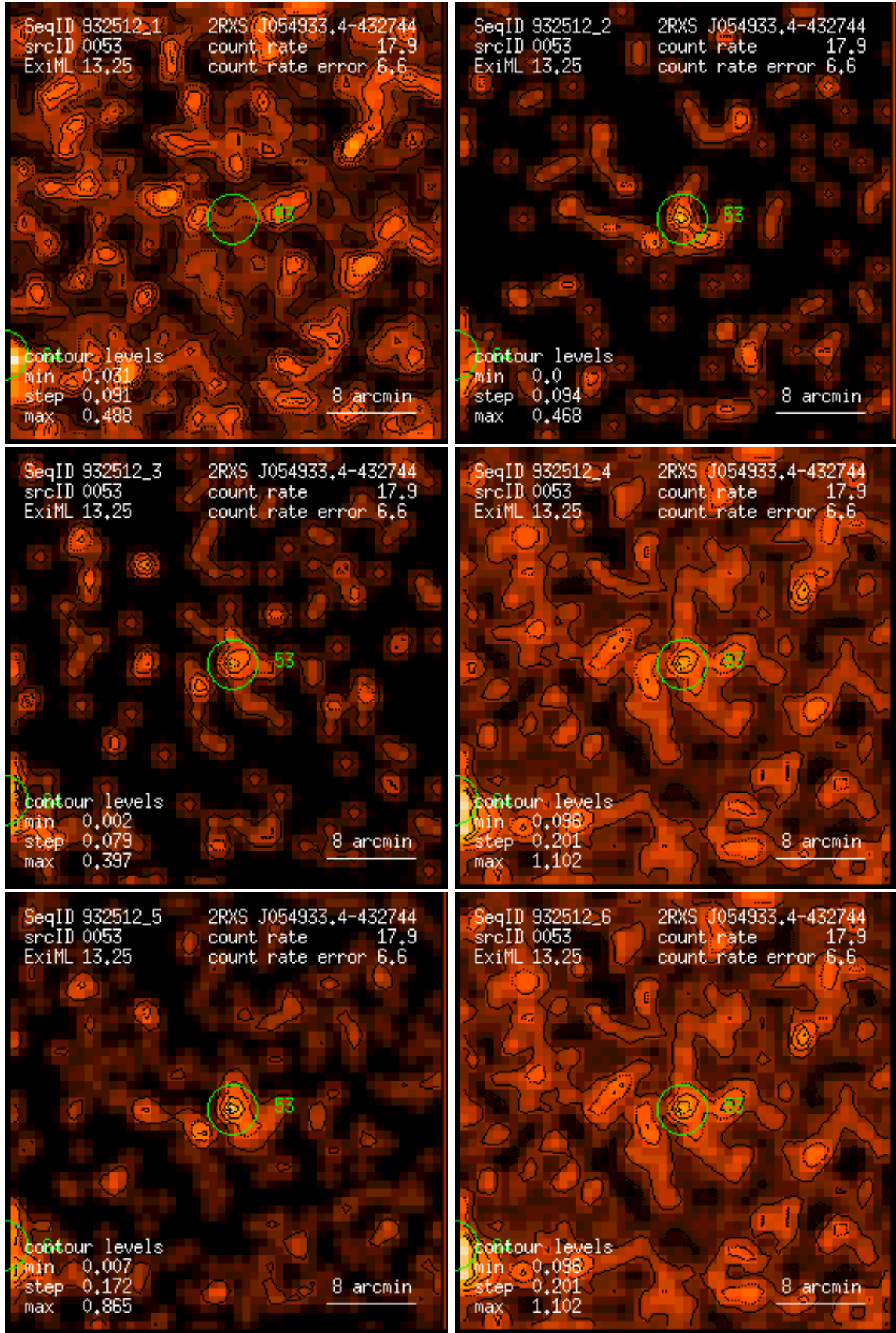
Figure 53: RASS 932512: detection 0053: band rate images, Gaussian filter: (1) PSPC channels 11 – 41, (2) 52 – 90, (3) 91 – 201, (4) 11 – 235, (5) 52 – 201, (6) 11 – 201. Broad band rates in counts/ks. Band rate contour levels in counts/ks/arcmin 2 .
