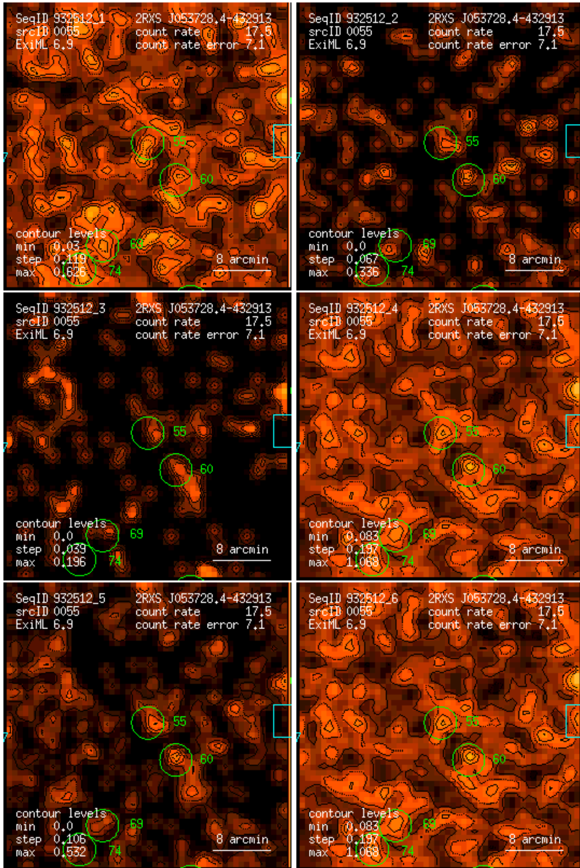
Figure 55: RASS 932512: detection 0055: band rate images, Gaussian filter: (1) PSPC channels 11 – 41, (2) 52 – 90, (3) 91 – 201, (4) 11 – 235, (5) 52 – 201, (6) 11 – 201. Broad band rates in counts/ks. Band rate contour levels in counts/ks/arcmin 2 .
