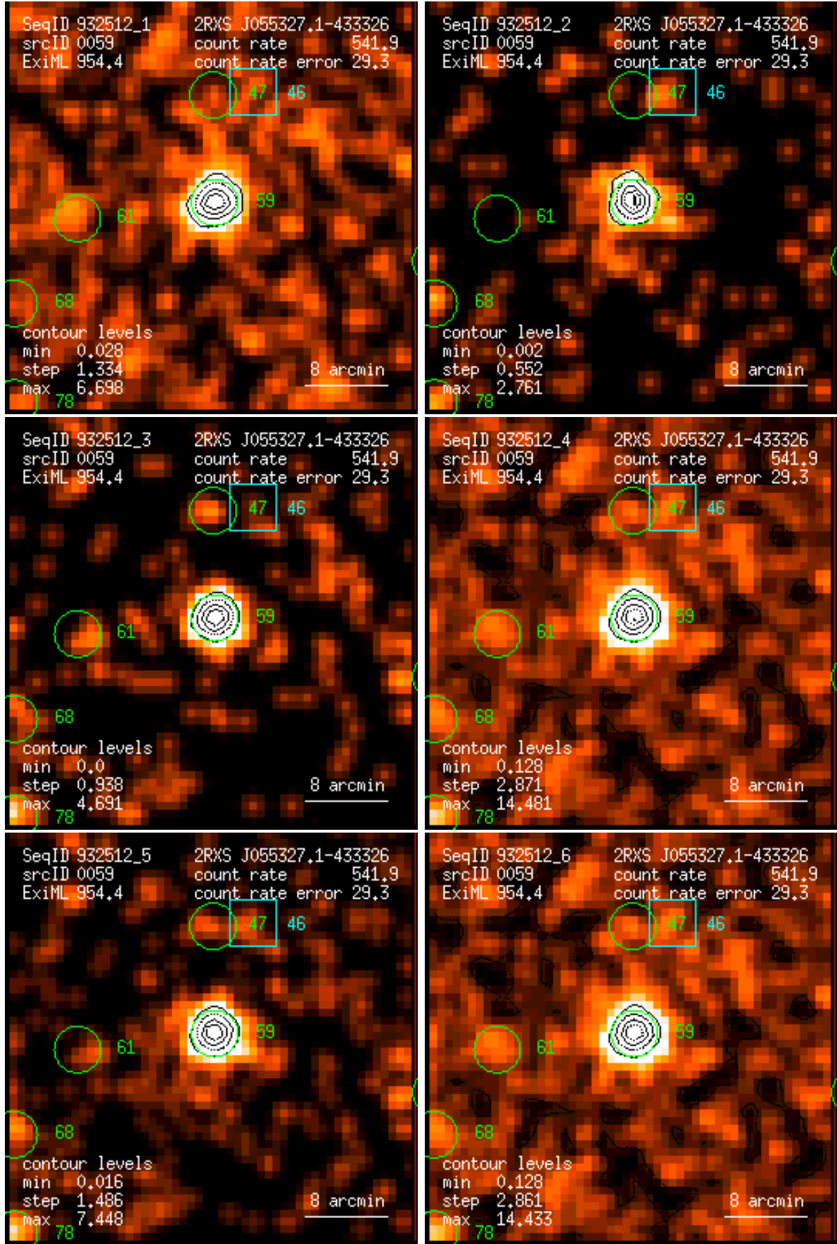
Figure 59: RASS 932512: detection 0059: band rate images, Gaussian filter: (1) PSPC channels 11 – 41, (2) 52 – 90, (3) 91 – 201, (4) 11 – 235, (5) 52 – 201, (6) 11 – 201. Broad band rates in counts/ks. Band rate contour levels in counts/ks/arcmin 2 .
