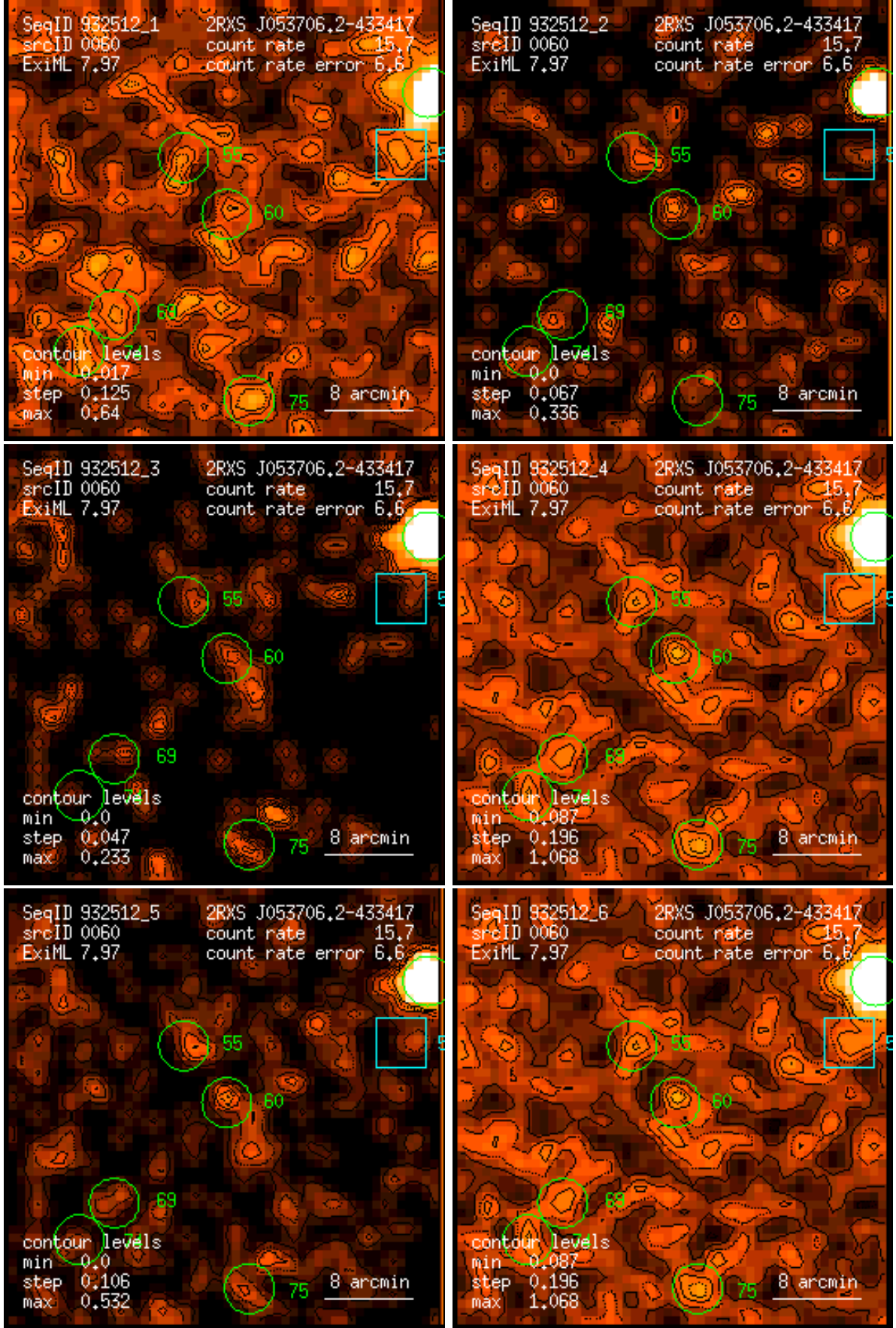
Figure 60: RASS 932512: detection 0060: band rate images, Gaussian filter: (1) PSPC channels 11 – 41, (2) 52 – 90, (3) 91 – 201, (4) 11 – 235, (5) 52 – 201, (6) 11 – 201. Broad band rates in counts/ks. Band rate contour levels in counts/ks/arcmin 2 .
