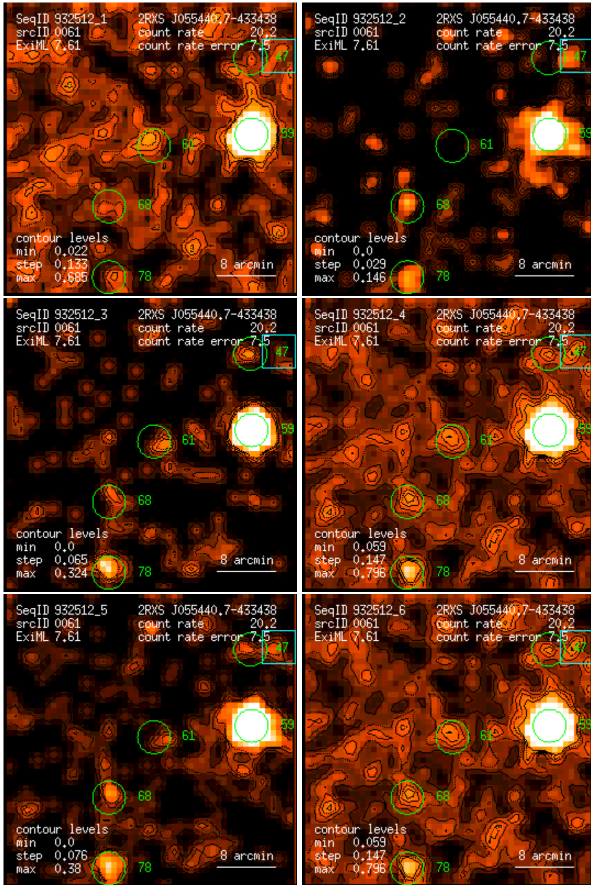
Figure 61: RASS 932512: detection 0061: band rate images, Gaussian filter: (1) PSPC channels 11 – 41, (2) 52 – 90, (3) 91 – 201, (4) 11 – 235, (5) 52 – 201, (6) 11 – 201. Broad band rates in counts/ks. Band rate contour levels in counts/ks/arcmin 2 .
