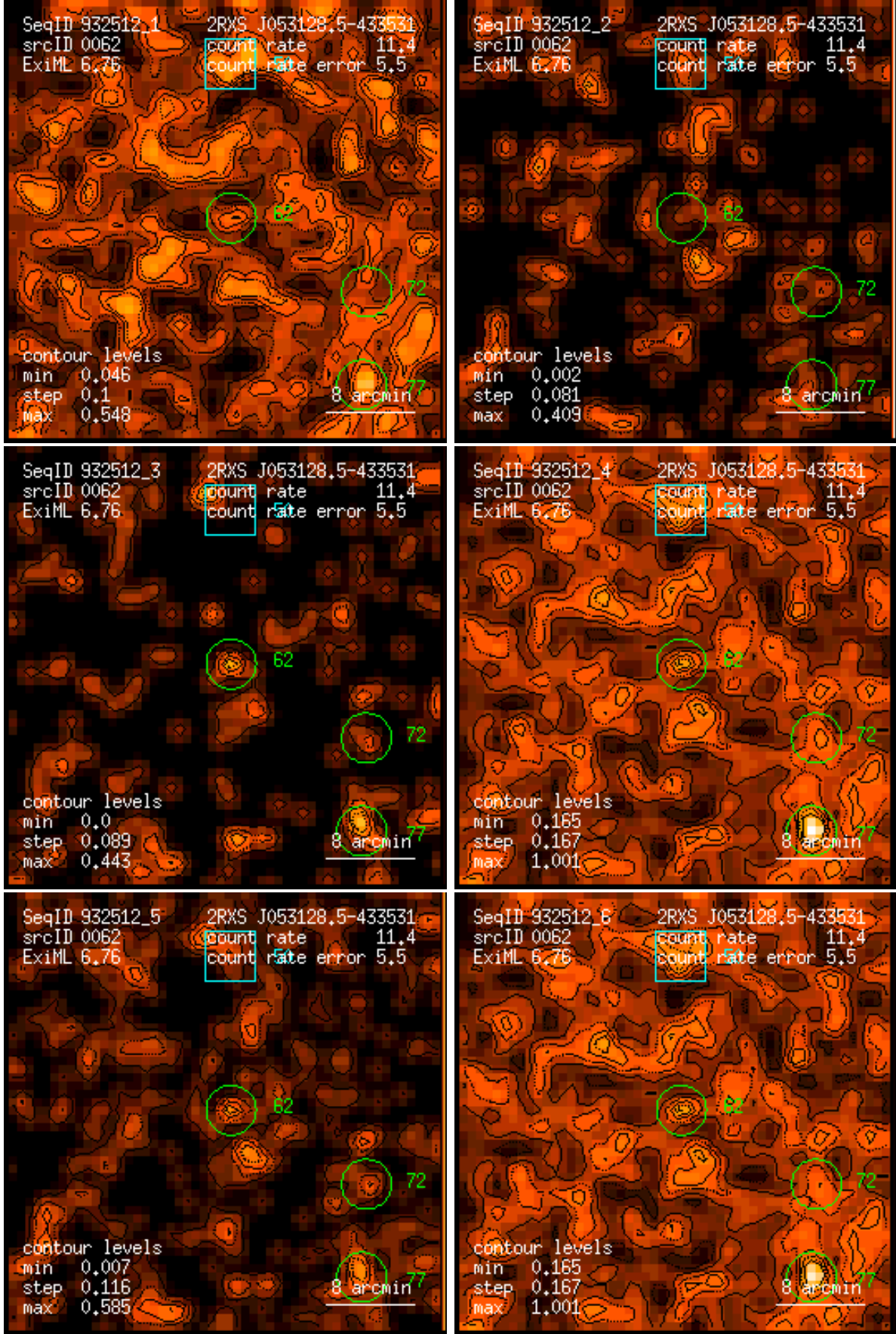
Figure 62: RASS 932512: detection 0062: band rate images, Gaussian filter: (1) PSPC channels 11 – 41, (2) 52 – 90, (3) 91 – 201, (4) 11 – 235, (5) 52 – 201, (6) 11 – 201. Broad band rates in counts/ks. Band rate contour levels in counts/ks/arcmin 2 .
