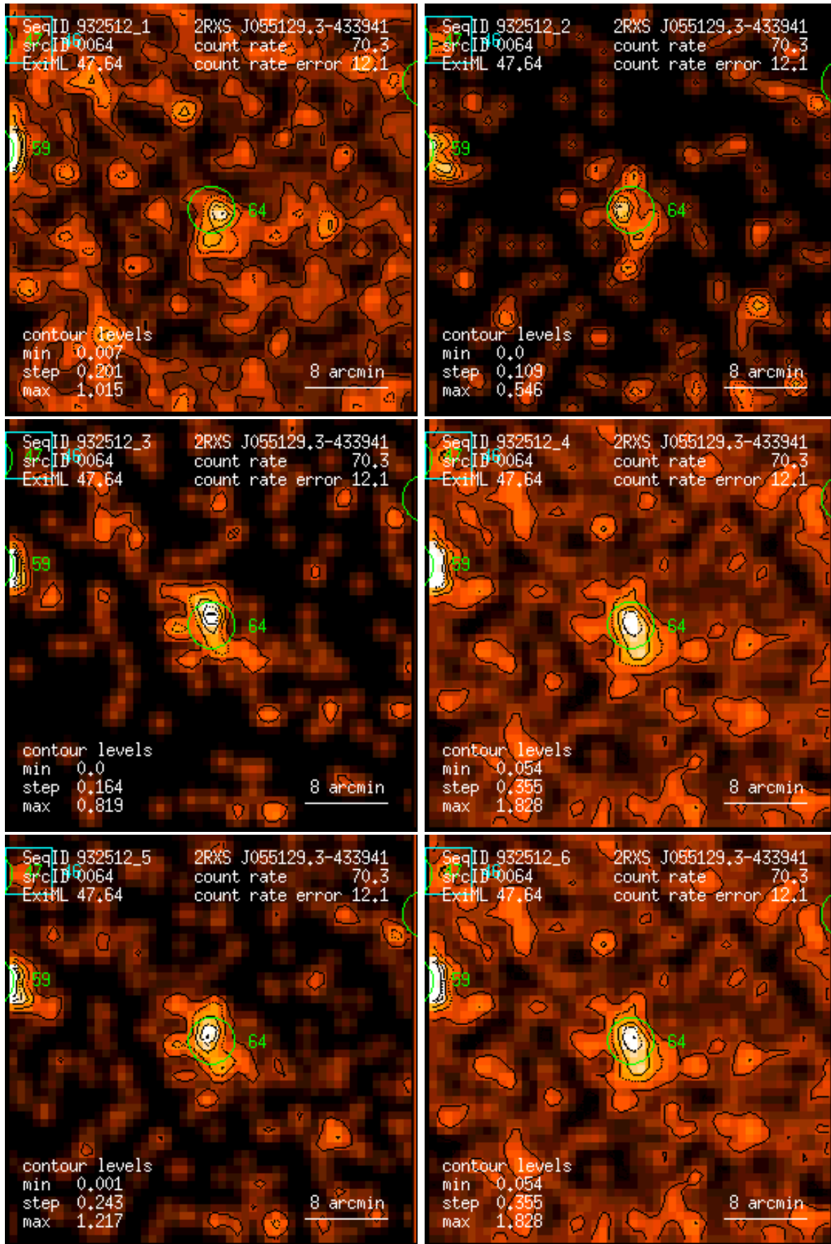
Figure 64: RASS 932512: detection 0064: band rate images, Gaussian filter: (1) PSPC channels 11 – 41, (2) 52 – 90, (3) 91 – 201, (4) 11 – 235, (5) 52 – 201, (6) 11 – 201. Broad band rates in counts/ks. Band rate contour levels in counts/ks/arcmin 2 .
