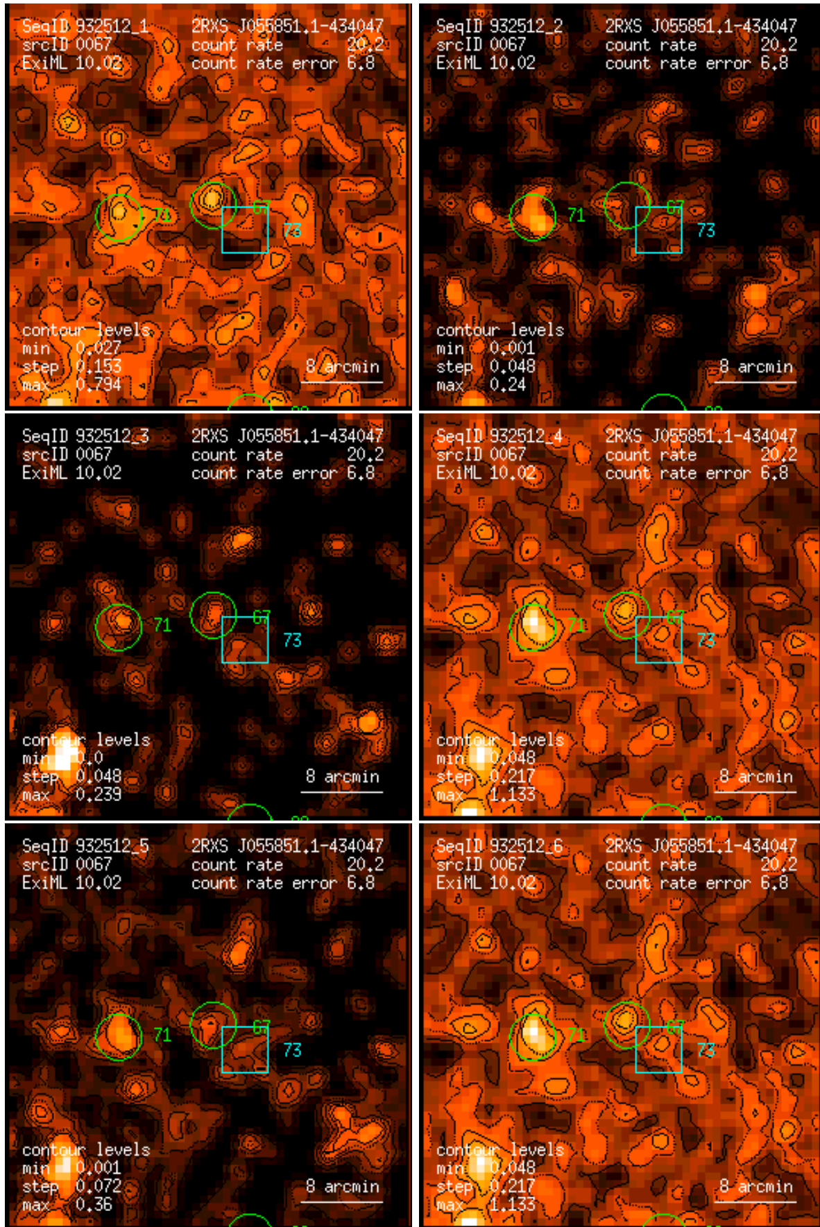
Figure 67: RASS 932512: detection 0067: band rate images, Gaussian filter: (1) PSPC channels 11 – 41, (2) 52 – 90, (3) 91 – 201, (4) 11 – 235, (5) 52 – 201, (6) 11 – 201. Broad band rates in counts/ks. Band rate contour levels in counts/ks/arcmin 2 .
