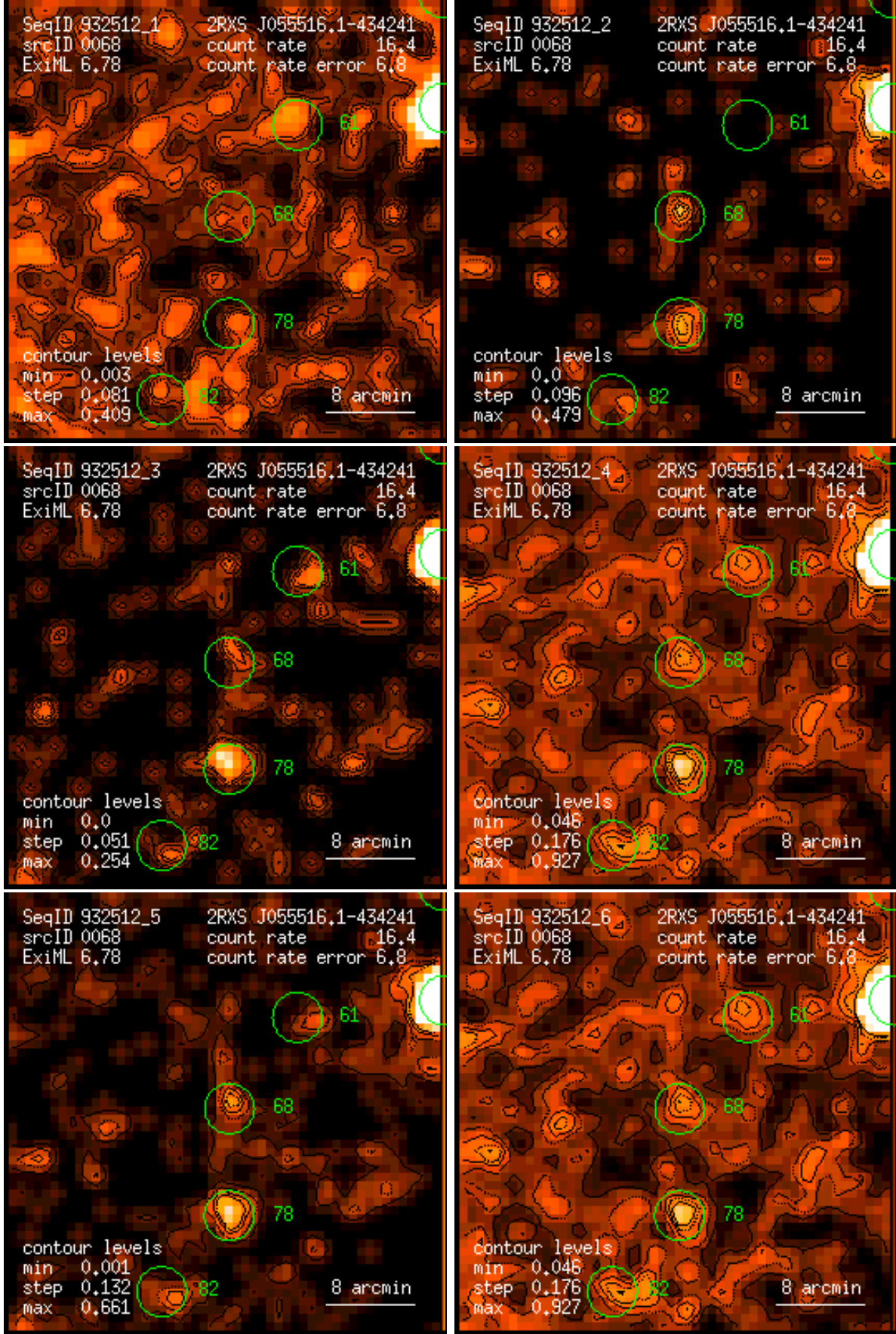
Figure 68: RASS 932512: detection 0068: band rate images, Gaussian filter: (1) PSPC channels 11 – 41, (2) 52 – 90, (3) 91 – 201, (4) 11 – 235, (5) 52 – 201, (6) 11 – 201. Broad band rates in counts/ks. Band rate contour levels in counts/ks/arcmin 2 .
