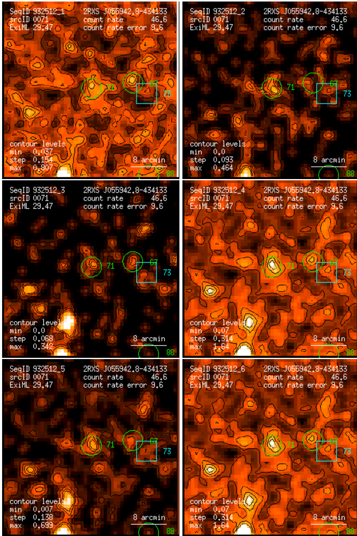
Figure 71: RASS 932512: detection 0071: band rate images, Gaussian filter: (1) PSPC channels 11 – 41, (2) 52 – 90, (3) 91 – 201, (4) 11 – 235, (5) 52 – 201, (6) 11 – 201. Broad band rates in counts/ks. Band rate contour levels in counts/ks/arcmin 2 .
