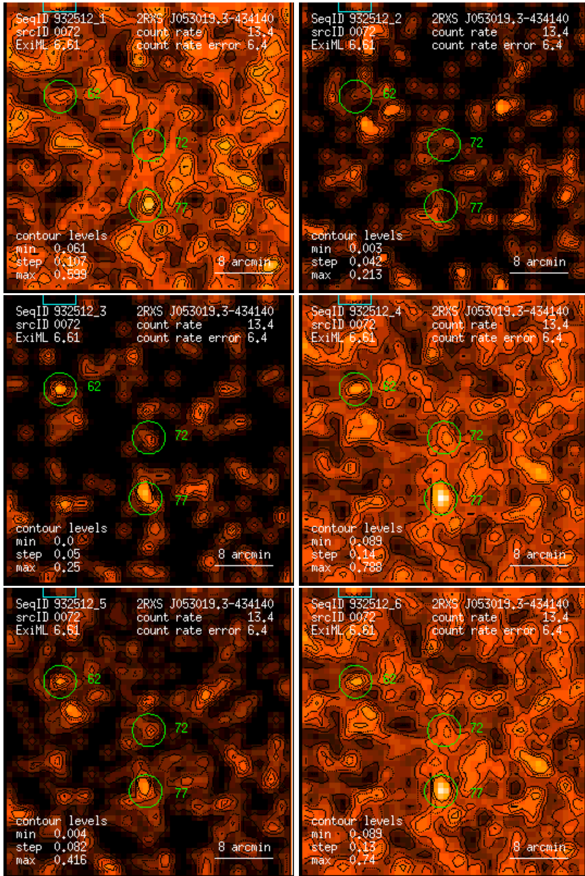
Figure 72: RASS 932512: detection 0072: band rate images, Gaussian filter: (1) PSPC channels 11 – 41, (2) 52 – 90, (3) 91 – 201, (4) 11 – 235, (5) 52 – 201, (6) 11 – 201. Broad band rates in counts/ks. Band rate contour levels in counts/ks/arcmin 2 .
