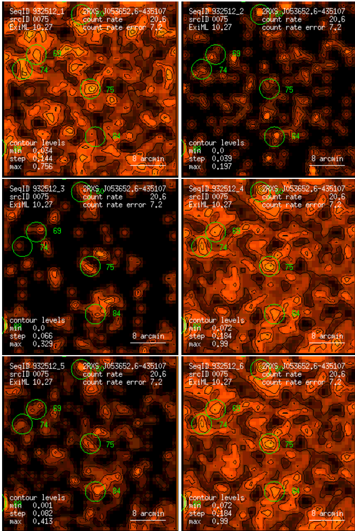
Figure 75: RASS 932512: detection 0075: band rate images, Gaussian filter: (1) PSPC channels 11 – 41, (2) 52 – 90, (3) 91 – 201, (4) 11 – 235, (5) 52 – 201, (6) 11 – 201. Broad band rates in counts/ks. Band rate contour levels in counts/ks/arcmin 2 .
