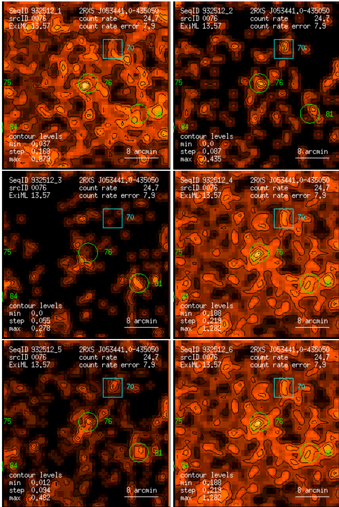
Figure 76: RASS 932512: detection 0076: band rate images, Gaussian filter: (1) PSPC channels 11 – 41, (2) 52 – 90, (3) 91 – 201, (4) 11 – 235, (5) 52 – 201, (6) 11 – 201. Broad band rates in counts/ks. Band rate contour levels in counts/ks/arcmin 2 .
