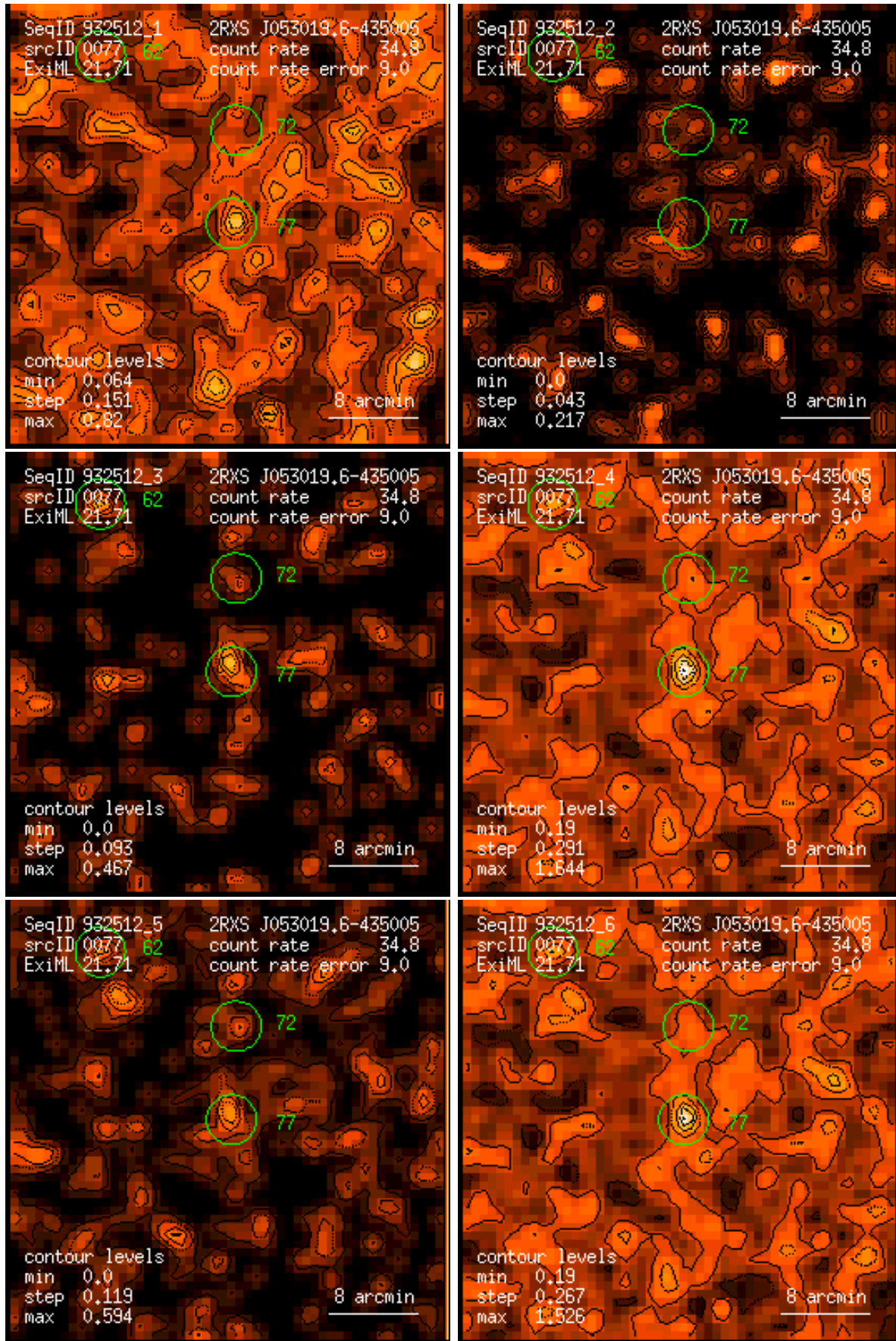
Figure 77: RASS 932512: detection 0077: band rate images, Gaussian filter: (1) PSPC channels 11 – 41, (2) 52 – 90, (3) 91 – 201, (4) 11 – 235, (5) 52 – 201, (6) 11 – 201. Broad band rates in counts/ks. Band rate contour levels in counts/ks/arcmin 2 .
