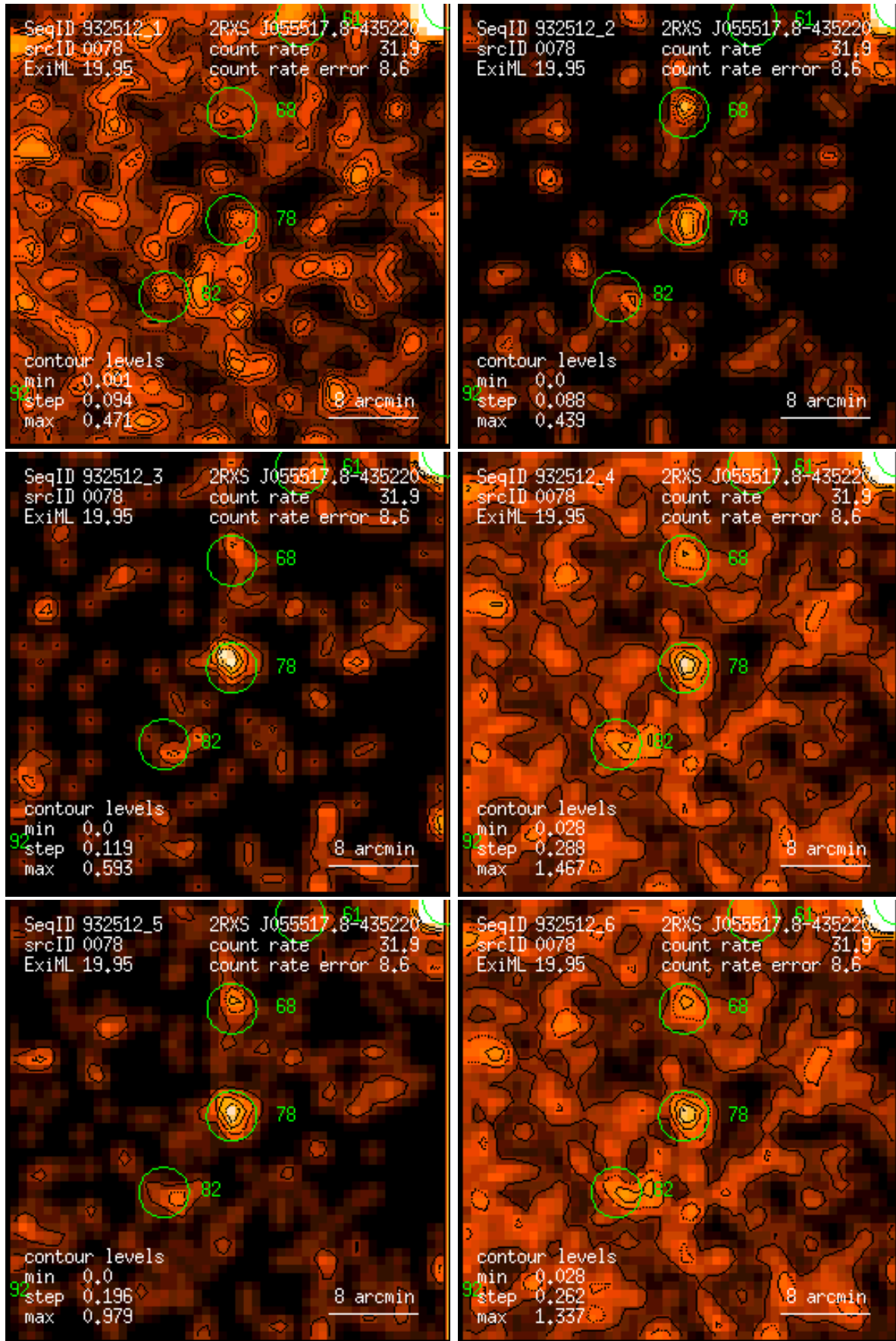
Figure 78: RASS 932512: detection 0078: band rate images, Gaussian filter: (1) PSPC channels 11 – 41, (2) 52 – 90, (3) 91 – 201, (4) 11 – 235, (5) 52 – 201, (6) 11 – 201. Broad band rates in counts/ks. Band rate contour levels in counts/ks/arcmin 2 .
