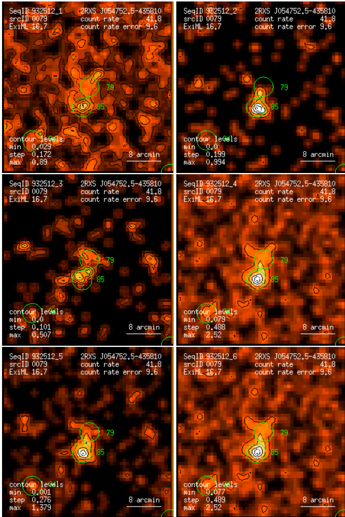
Figure 79: RASS 932512: detection 0079: band rate images, Gaussian filter: (1) PSPC channels 11 – 41, (2) 52 – 90, (3) 91 – 201, (4) 11 – 235, (5) 52 – 201, (6) 11 – 201. Broad band rates in counts/ks. Band rate contour levels in counts/ks/arcmin 2 .
