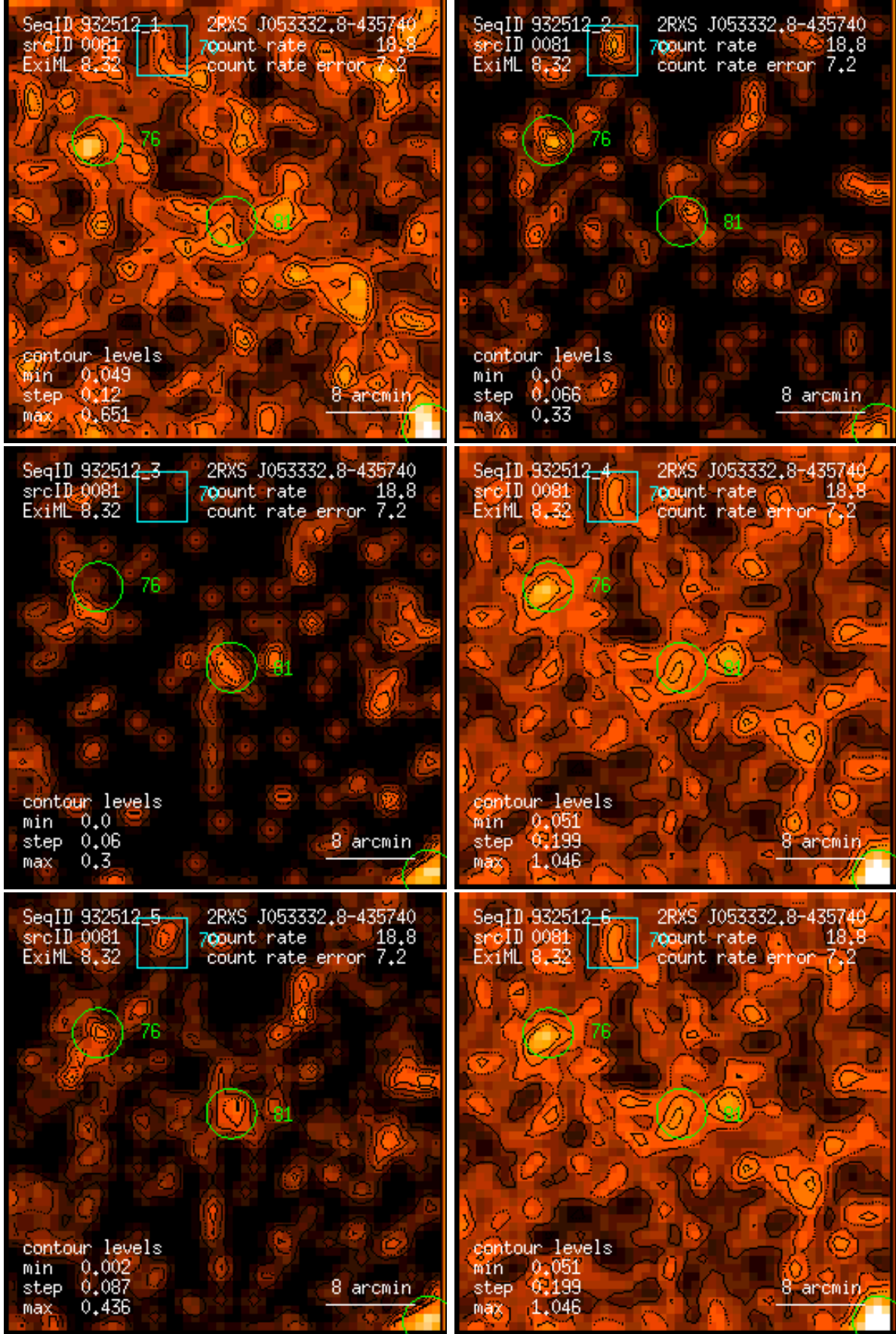
Figure 81: RASS 932512: detection 0081: band rate images, Gaussian filter: (1) PSPC channels 11 – 41, (2) 52 – 90, (3) 91 – 201, (4) 11 – 235, (5) 52 – 201, (6) 11 – 201. Broad band rates in counts/ks. Band rate contour levels in counts/ks/arcmin 2 .
