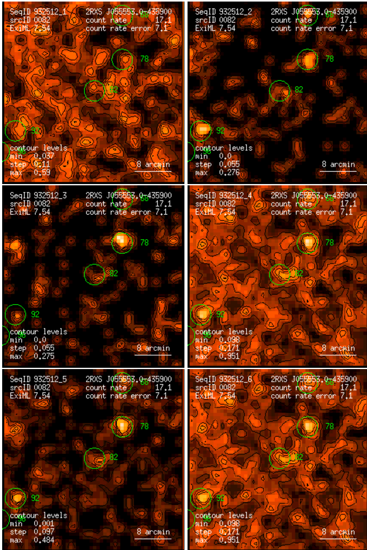
Figure 82: RASS 932512: detection 0082: band rate images, Gaussian filter: (1) PSPC channels 11 – 41, (2) 52 – 90, (3) 91 – 201, (4) 11 – 235, (5) 52 – 201, (6) 11 – 201. Broad band rates in counts/ks. Band rate contour levels in counts/ks/arcmin 2 .
