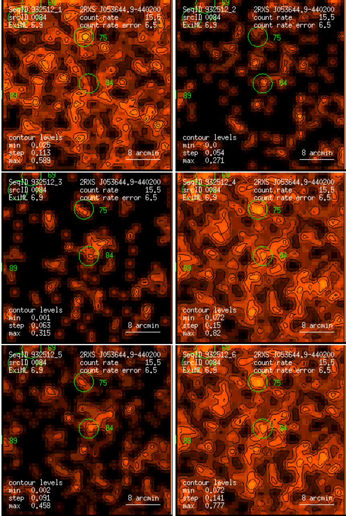
Figure 84: RASS 932512: detection 0084: band rate images, Gaussian filter: (1) PSPC channels 11 – 41, (2) 52 – 90, (3) 91 – 201, (4) 11 – 235, (5) 52 – 201, (6) 11 – 201. Broad band rates in counts/ks. Band rate contour levels in counts/ks/arcmin 2 .
