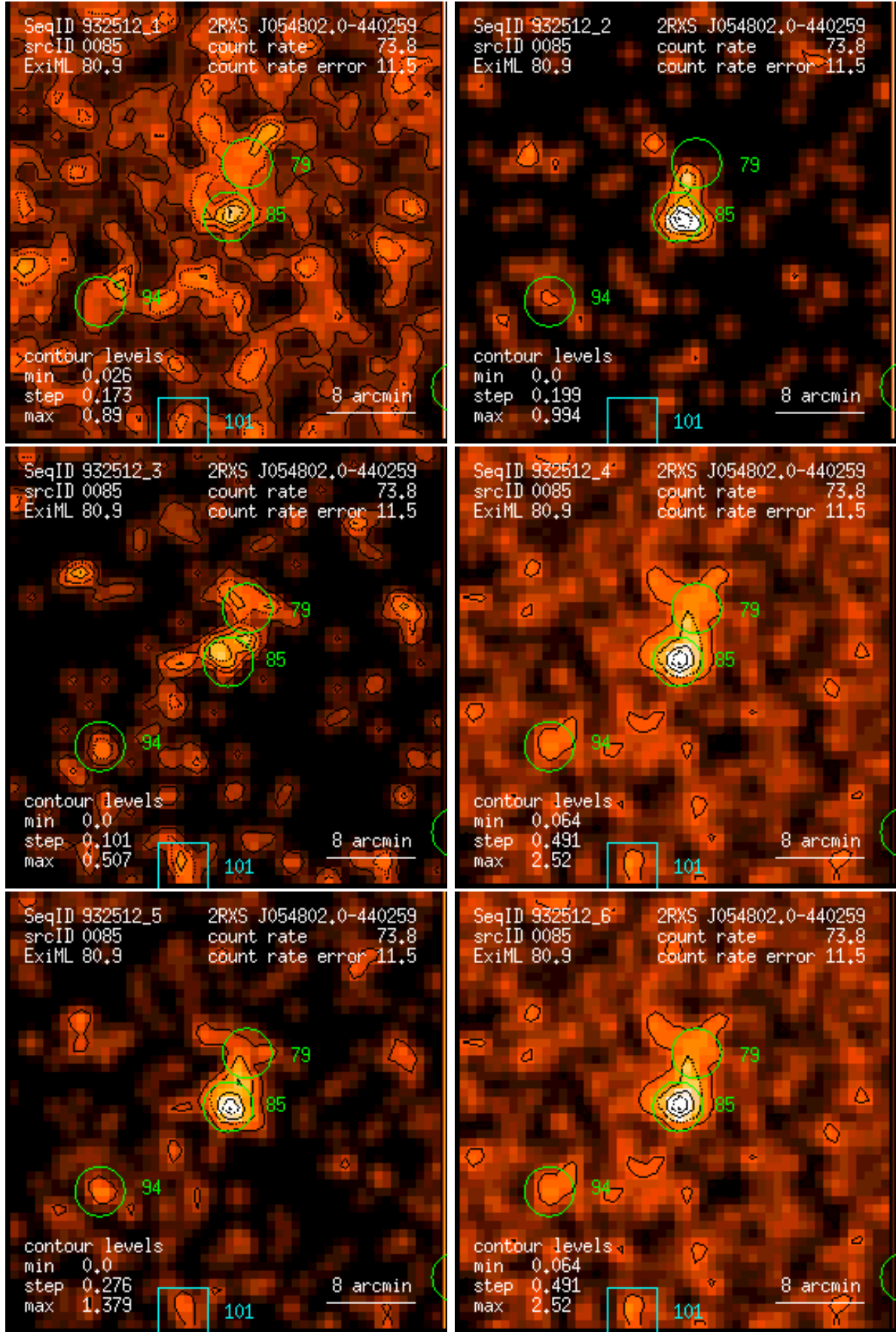
Figure 85: RASS 932512: detection 0085: band rate images, Gaussian filter: (1) PSPC channels 11 – 41, (2) 52 – 90, (3) 91 – 201, (4) 11 – 235, (5) 52 – 201, (6) 11 – 201. Broad band rates in counts/ks. Band rate contour levels in counts/ks/arcmin 2 .
