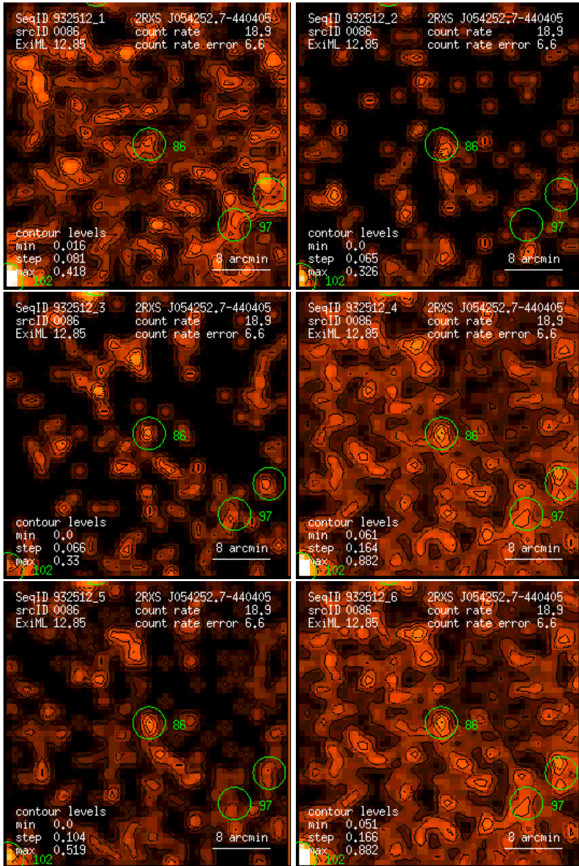
Figure 86: RASS 932512: detection 0086: band rate images, Gaussian filter: (1) PSPC channels 11 – 41, (2) 52 – 90, (3) 91 – 201, (4) 11 – 235, (5) 52 – 201, (6) 11 – 201. Broad band rates in counts/ks. Band rate contour levels in counts/ks/arcmin 2 .
