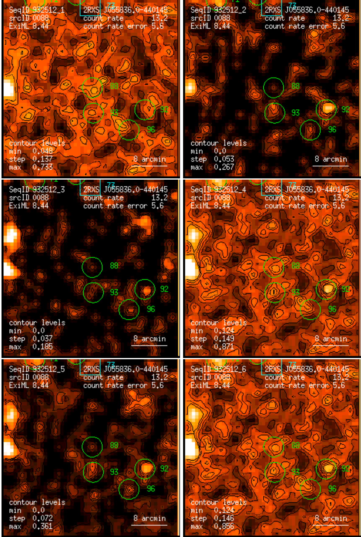
Figure 88: RASS 932512: detection 0088: band rate images, Gaussian filter: (1) PSPC channels 11 – 41, (2) 52 – 90, (3) 91 – 201, (4) 11 – 235, (5) 52 – 201, (6) 11 – 201. Broad band rates in counts/ks. Band rate contour levels in counts/ks/arcmin 2 .
