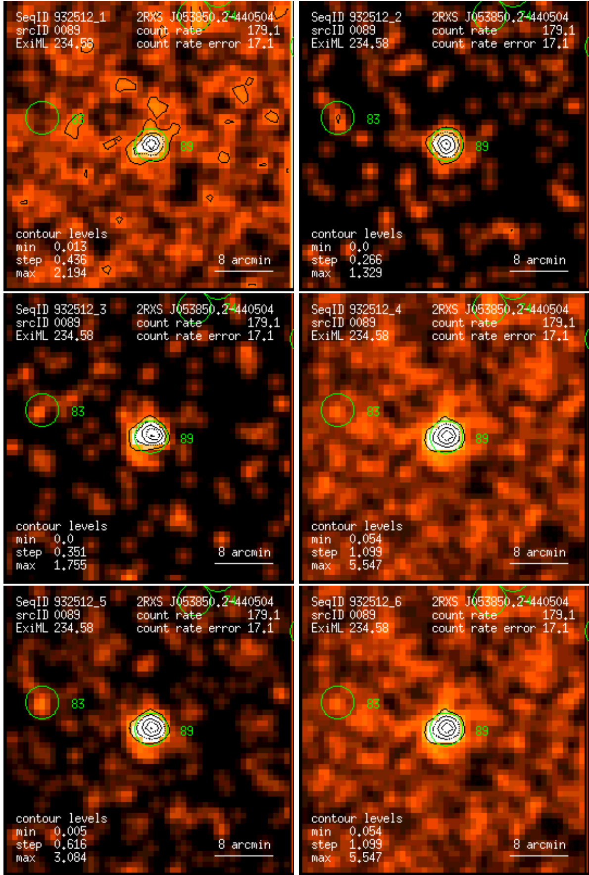
Figure 89: RASS 932512: detection 0089: band rate images, Gaussian filter: (1) PSPC channels 11 – 41, (2) 52 – 90, (3) 91 – 201, (4) 11 – 235, (5) 52 – 201, (6) 11 – 201. Broad band rates in counts/ks. Band rate contour levels in counts/ks/arcmin 2 .
