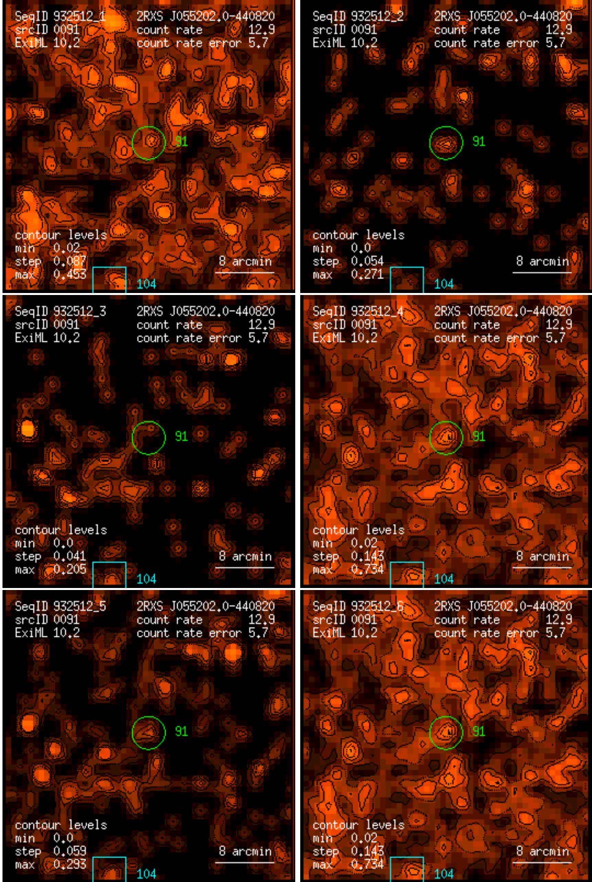
Figure 91: RASS 932512: detection 0091: band rate images, Gaussian filter: (1) PSPC channels 11 – 41, (2) 52 – 90, (3) 91 – 201, (4) 11 – 235, (5) 52 – 201, (6) 11 – 201. Broad band rates in counts/ks. Band rate contour levels in counts/ks/arcmin 2 .
