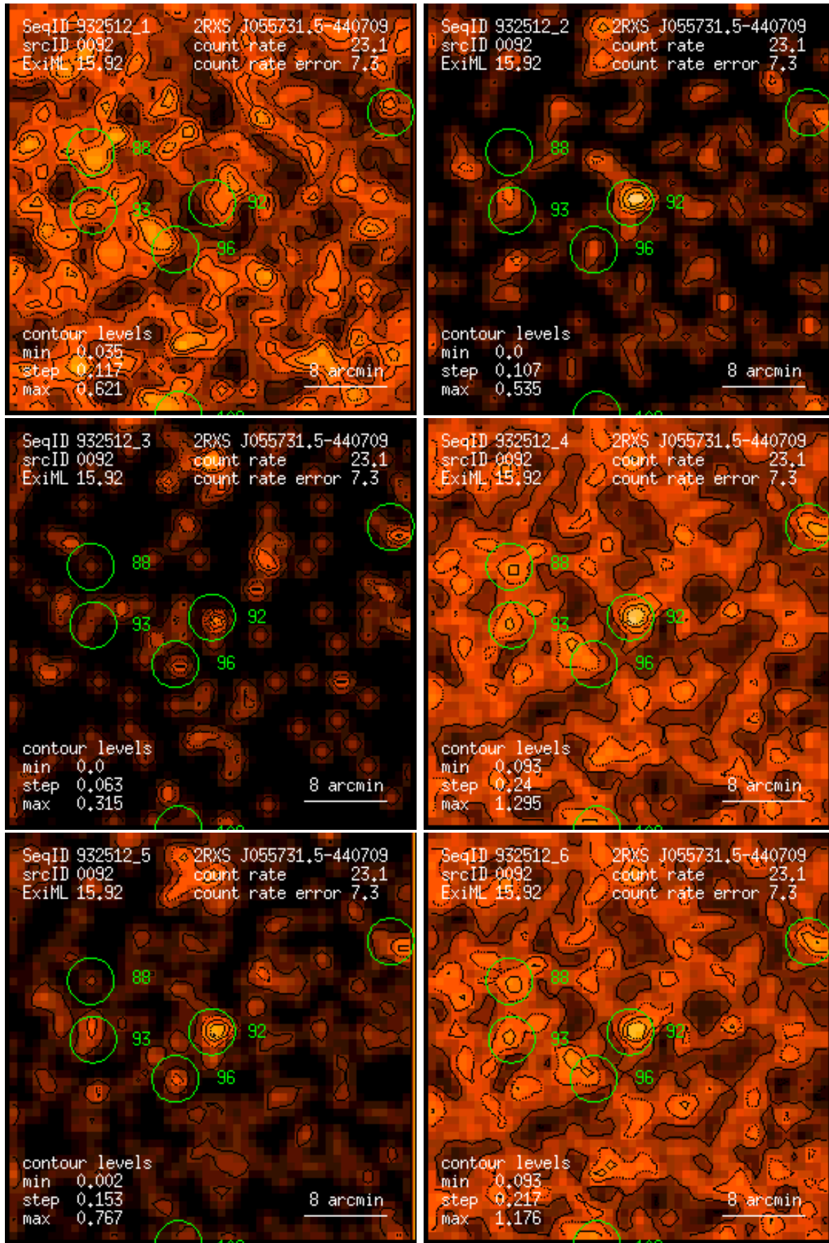
Figure 92: RASS 932512: detection 0092: band rate images, Gaussian filter: (1) PSPC channels 11 – 41, (2) 52 – 90, (3) 91 – 201, (4) 11 – 235, (5) 52 – 201, (6) 11 – 201. Broad band rates in counts/ks. Band rate contour levels in counts/ks/arcmin 2 .
