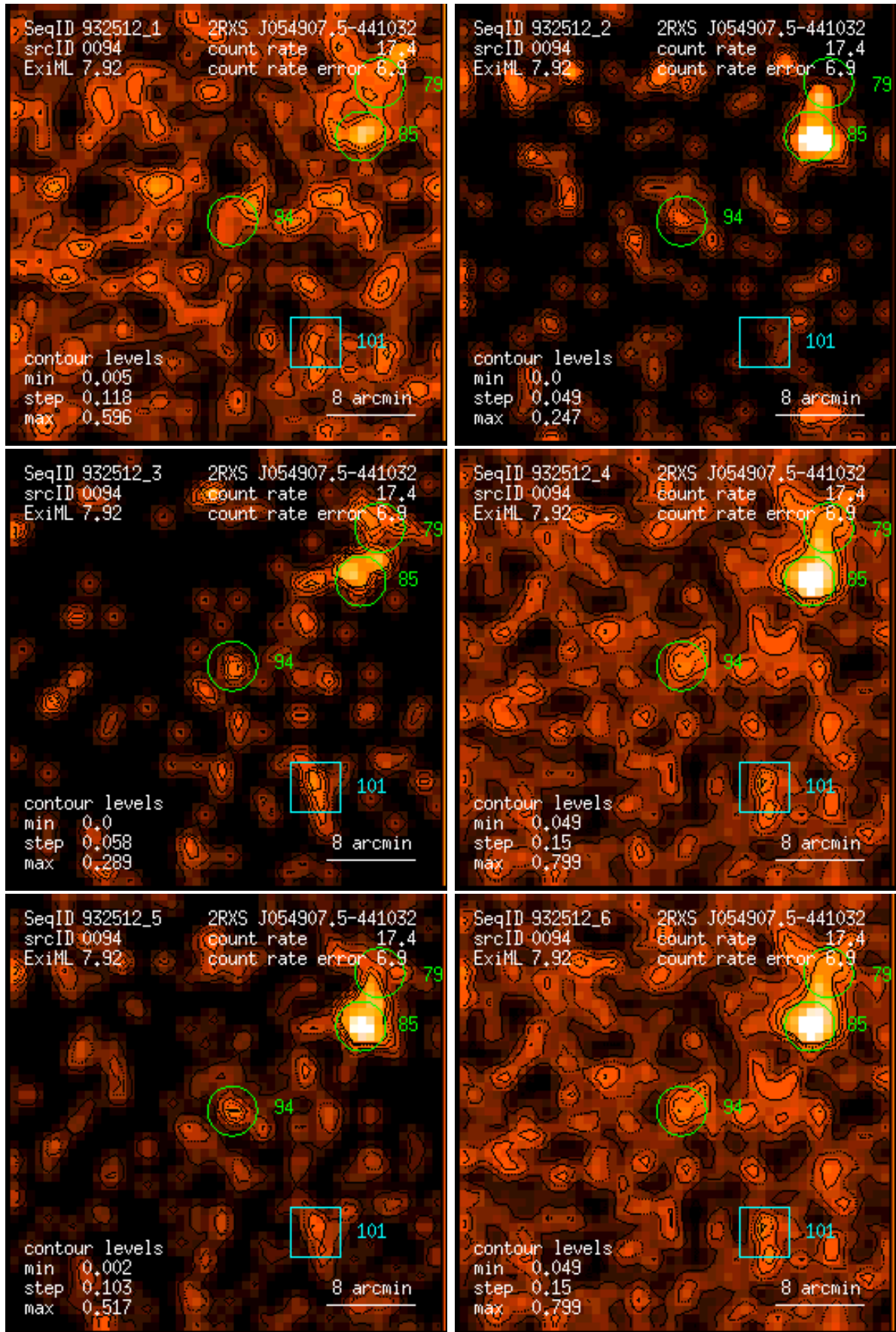
Figure 94: RASS 932512: detection 0094: band rate images, Gaussian filter: (1) PSPC channels 11 – 41, (2) 52 – 90, (3) 91 – 201, (4) 11 – 235, (5) 52 – 201, (6) 11 – 201. Broad band rates in counts/ks. Band rate contour levels in counts/ks/arcmin 2 .
