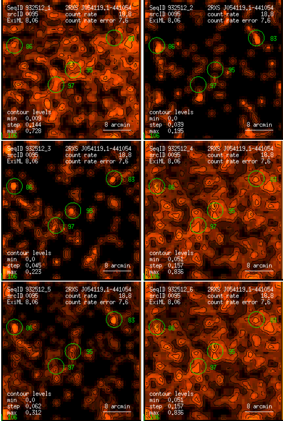
Figure 95: RASS 932512: detection 0095: band rate images, Gaussian filter: (1) PSPC channels 11 – 41, (2) 52 – 90, (3) 91 – 201, (4) 11 – 235, (5) 52 – 201, (6) 11 – 201. Broad band rates in counts/ks. Band rate contour levels in counts/ks/arcmin 2 .
