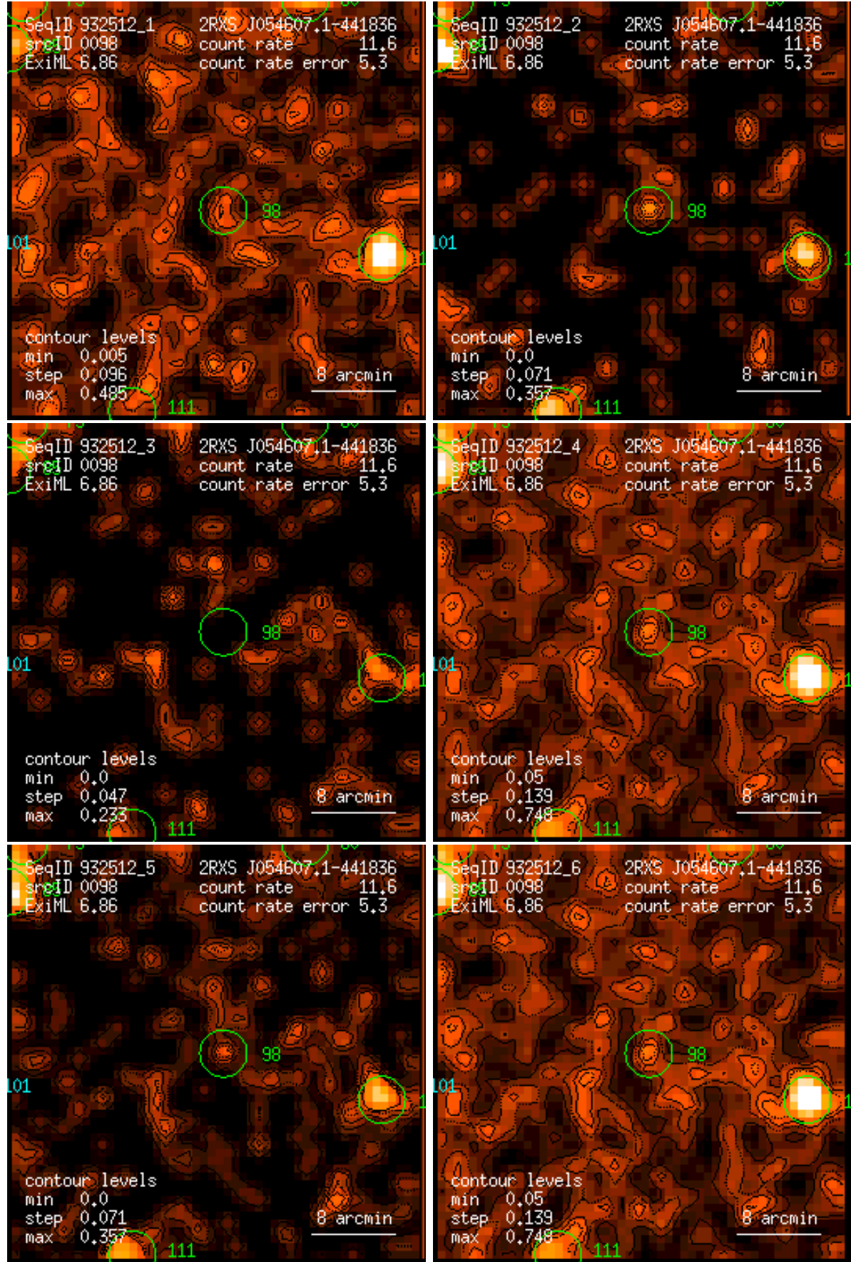
Figure 98: RASS 932512: detection 0098: band rate images, Gaussian filter: (1) PSPC channels 11 – 41, (2) 52 – 90, (3) 91 – 201, (4) 11 – 235, (5) 52 – 201, (6) 11 – 201. Broad band rates in counts/ks. Band rate contour levels in counts/ks/arcmin 2 .
