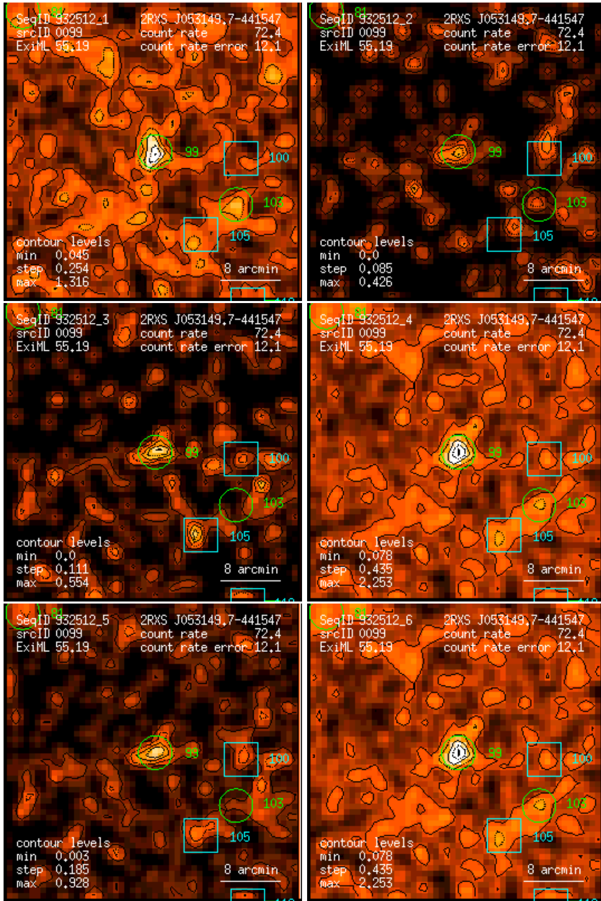
Figure 99: RASS 932512: detection 0099: band rate images, Gaussian filter: (1) PSPC channels 11 – 41, (2) 52 – 90, (3) 91 – 201, (4) 11 – 235, (5) 52 – 201, (6) 11 – 201. Broad band rates in counts/ks. Band rate contour levels in counts/ks/arcmin 2 .
