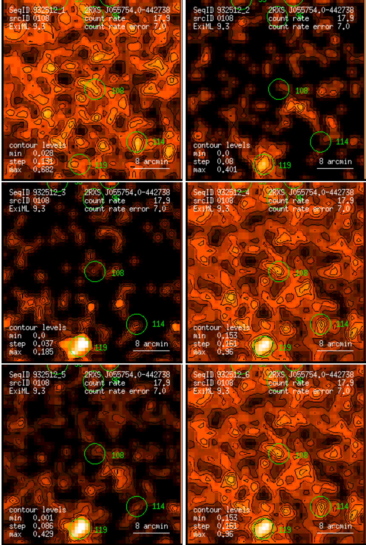
Figure 108: RASS 932512: detection 0108: band rate images, Gaussian filter: (1) PSPC channels 11 – 41, (2) 52 – 90, (3) 91 – 201, (4) 11 – 235, (5) 52 – 201, (6) 11 – 201. Broad band rates in counts/ks. Band rate contour levels in counts/ks/arcmin 2 .
