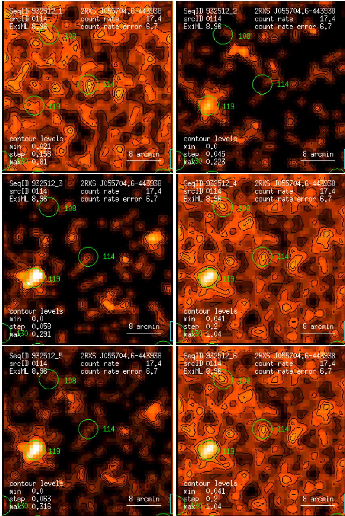
Figure 114: RASS 932512: detection 0114: band rate images, Gaussian filter: (1) PSPC channels 11 – 41, (2) 52 – 90, (3) 91 – 201, (4) 11 – 235, (5) 52 – 201, (6) 11 – 201. Broad band rates in counts/ks. Band rate contour levels in counts/ks/arcmin 2 .
