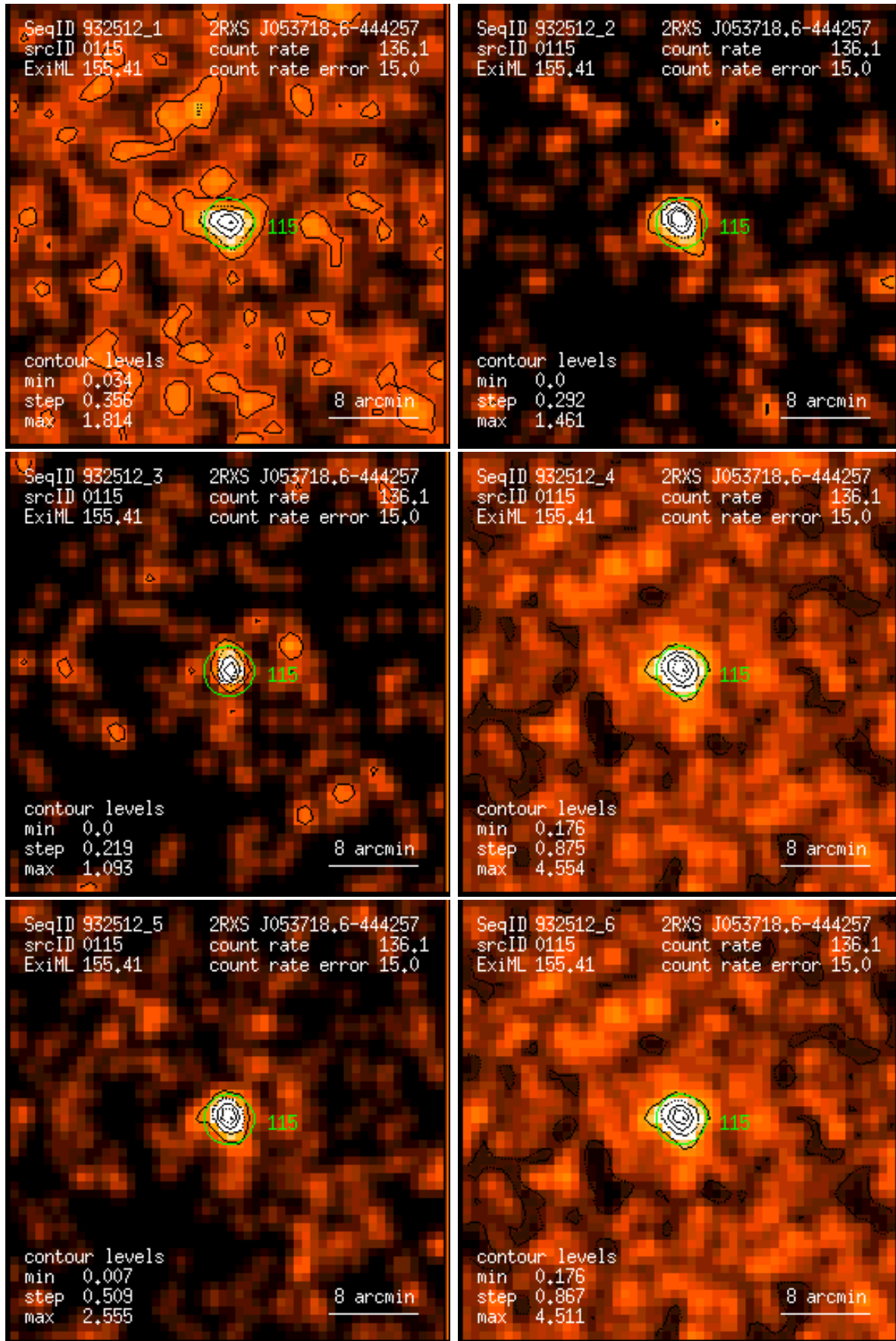
Figure 115: RASS 932512: detection 0115: band rate images, Gaussian filter: (1) PSPC channels 11 – 41, (2) 52 – 90, (3) 91 – 201, (4) 11 – 235, (5) 52 – 201, (6) 11 – 201. Broad band rates in counts/ks. Band rate contour levels in counts/ks/arcmin 2 .
