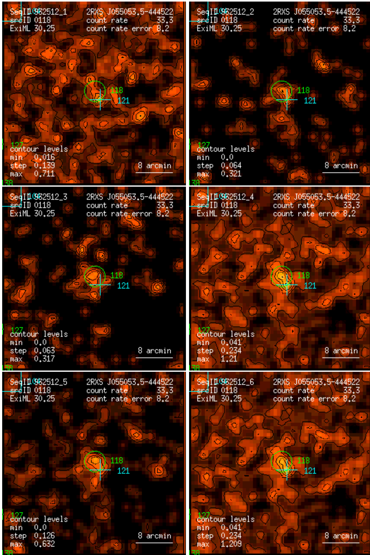
Figure 118: RASS 932512: detection 0118: band rate images, Gaussian filter: (1) PSPC channels 11 – 41, (2) 52 – 90, (3) 91 – 201, (4) 11 – 235, (5) 52 – 201, (6) 11 – 201. Broad band rates in counts/ks. Band rate contour levels in counts/ks/arcmin 2 .
