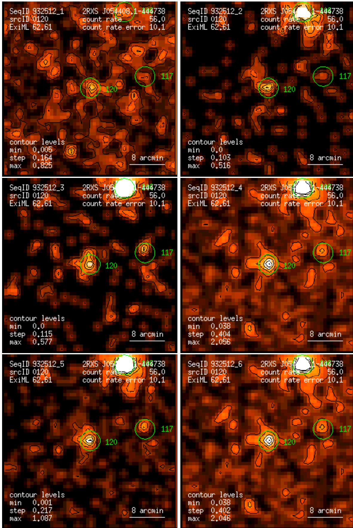
Figure 120: RASS 932512: detection 0120: band rate images, Gaussian filter: (1) PSPC channels 11 – 41, (2) 52 – 90, (3) 91 – 201, (4) 11 – 235, (5) 52 – 201, (6) 11 – 201. Broad band rates in counts/ks. Band rate contour levels in counts/ks/arcmin 2 .
