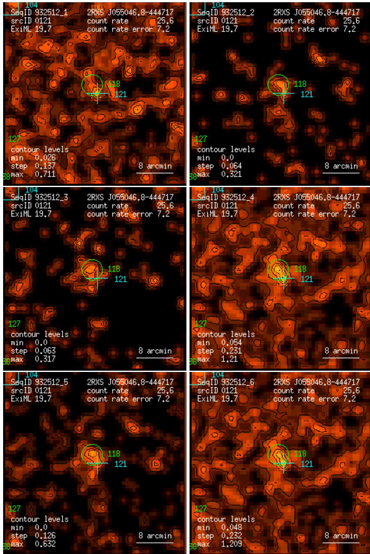
Figure 121: RASS 932512: detection 0121: band rate images, Gaussian filter: (1) PSPC channels 11 – 41, (2) 52 – 90, (3) 91 – 201, (4) 11 – 235, (5) 52 – 201, (6) 11 – 201. Broad band rates in counts/ks. Band rate contour levels in counts/ks/arcmin 2 .
