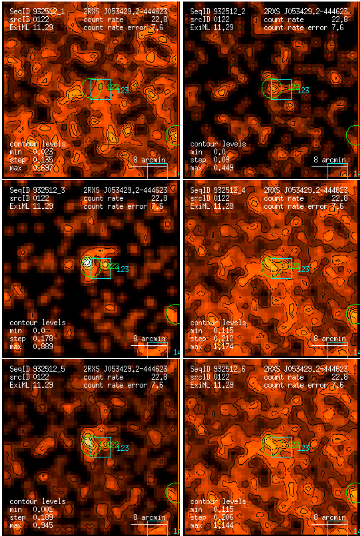
Figure 122: RASS 932512: detection 0122: band rate images, Gaussian filter: (1) PSPC channels 11 – 41, (2) 52 – 90, (3) 91 – 201, (4) 11 – 235, (5) 52 – 201, (6) 11 – 201. Broad band rates in counts/ks. Band rate contour levels in counts/ks/arcmin 2 .
