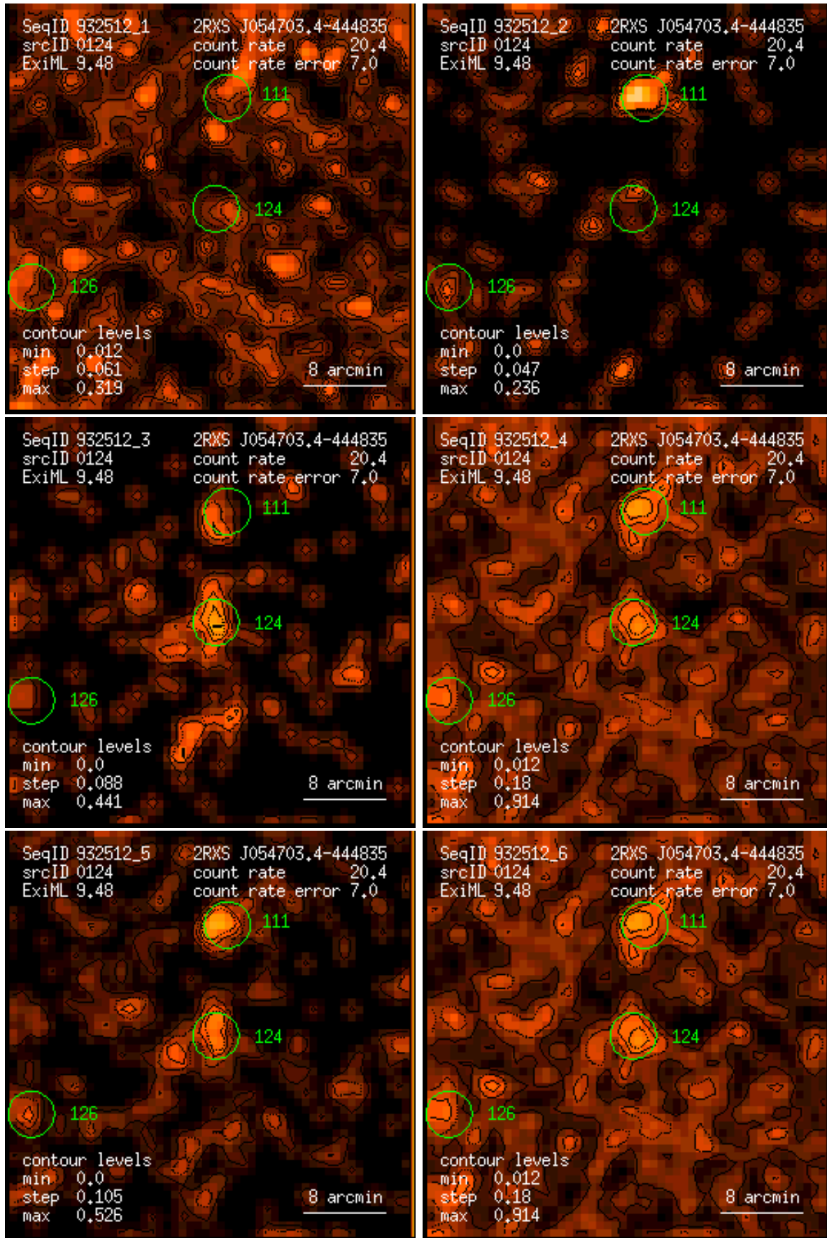
Figure 124: RASS 932512: detection 0124: band rate images, Gaussian filter: (1) PSPC channels 11 – 41, (2) 52 – 90, (3) 91 – 201, (4) 11 – 235, (5) 52 – 201, (6) 11 – 201. Broad band rates in counts/ks. Band rate contour levels in counts/ks/arcmin 2 .
