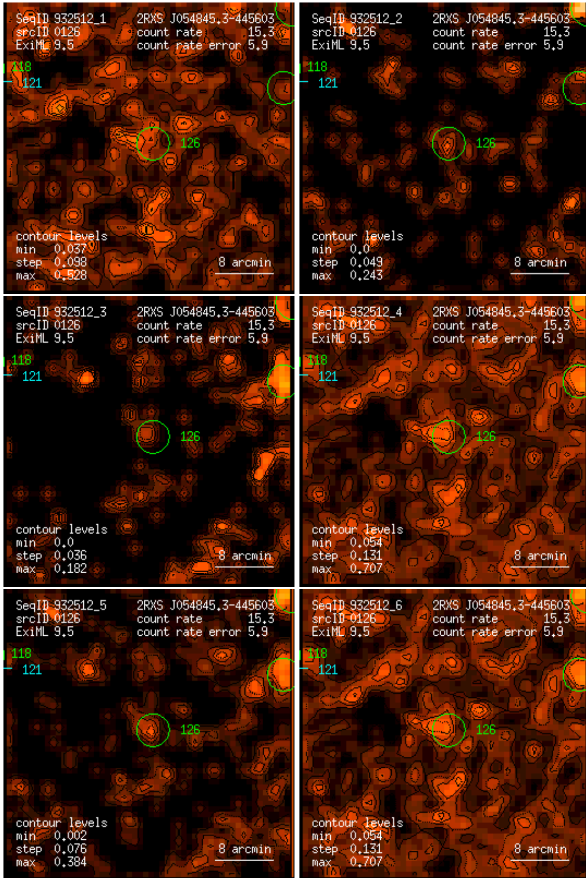
Figure 126: RASS 932512: detection 0126: band rate images, Gaussian filter: (1) PSPC channels 11 – 41, (2) 52 – 90, (3) 91 – 201, (4) 11 – 235, (5) 52 – 201, (6) 11 – 201. Broad band rates in counts/ks. Band rate contour levels in counts/ks/arcmin 2 .
