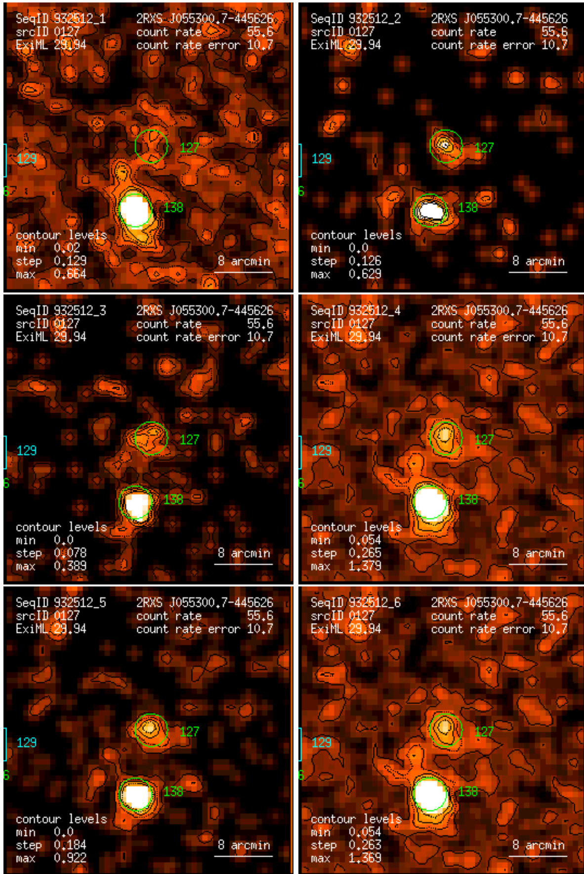
Figure 127: RASS 932512: detection 0127: band rate images, Gaussian filter: (1) PSPC channels 11 – 41, (2) 52 – 90, (3) 91 – 201, (4) 11 – 235, (5) 52 – 201, (6) 11 – 201. Broad band rates in counts/ks. Band rate contour levels in counts/ks/arcmin 2 .
