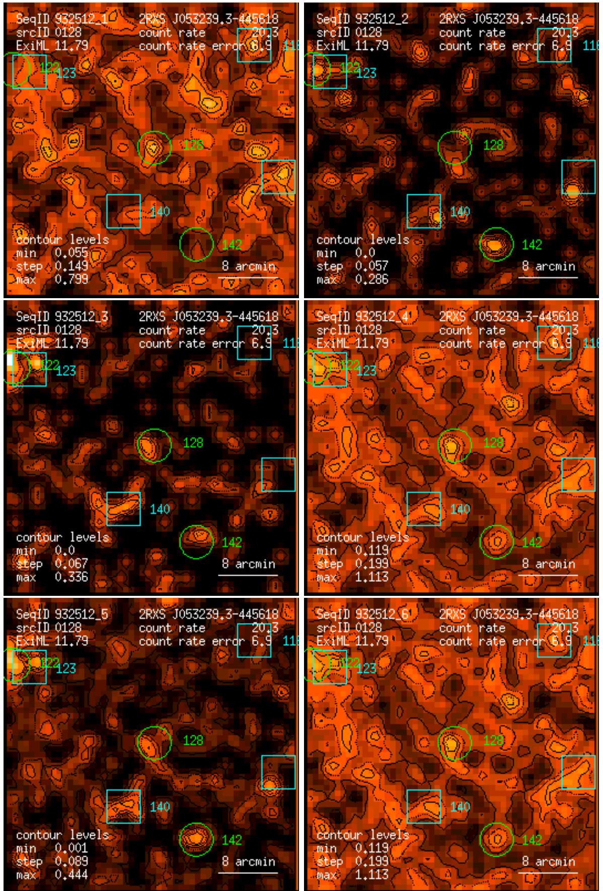
Figure 128: RASS 932512: detection 0128: band rate images, Gaussian filter: (1) PSPC channels 11 – 41, (2) 52 – 90, (3) 91 – 201, (4) 11 – 235, (5) 52 – 201, (6) 11 – 201. Broad band rates in counts/ks. Band rate contour levels in counts/ks/arcmin 2 .
