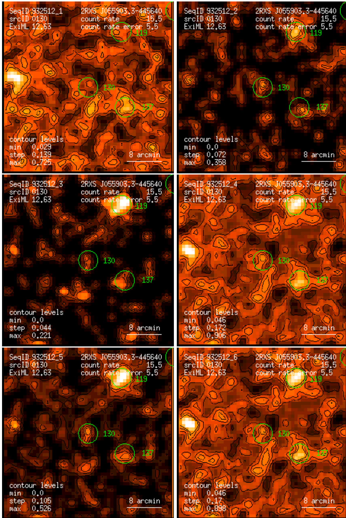
Figure 130: RASS 932512: detection 0130: band rate images, Gaussian filter: (1) PSPC channels 11 – 41, (2) 52 – 90, (3) 91 – 201, (4) 11 – 235, (5) 52 – 201, (6) 11 – 201. Broad band rates in counts/ks. Band rate contour levels in counts/ks/arcmin 2 .
