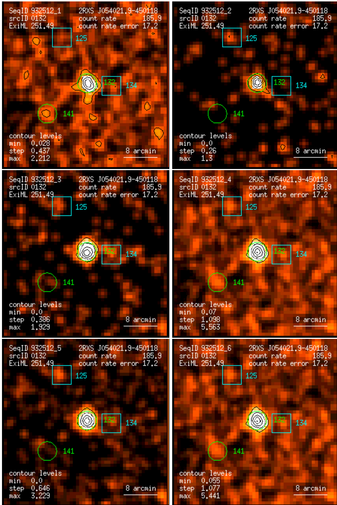
Figure 132: RASS 932512: detection 0132: band rate images, Gaussian filter: (1) PSPC channels 11 – 41, (2) 52 – 90, (3) 91 – 201, (4) 11 – 235, (5) 52 – 201, (6) 11 – 201. Broad band rates in counts/ks. Band rate contour levels in counts/ks/arcmin 2 .
