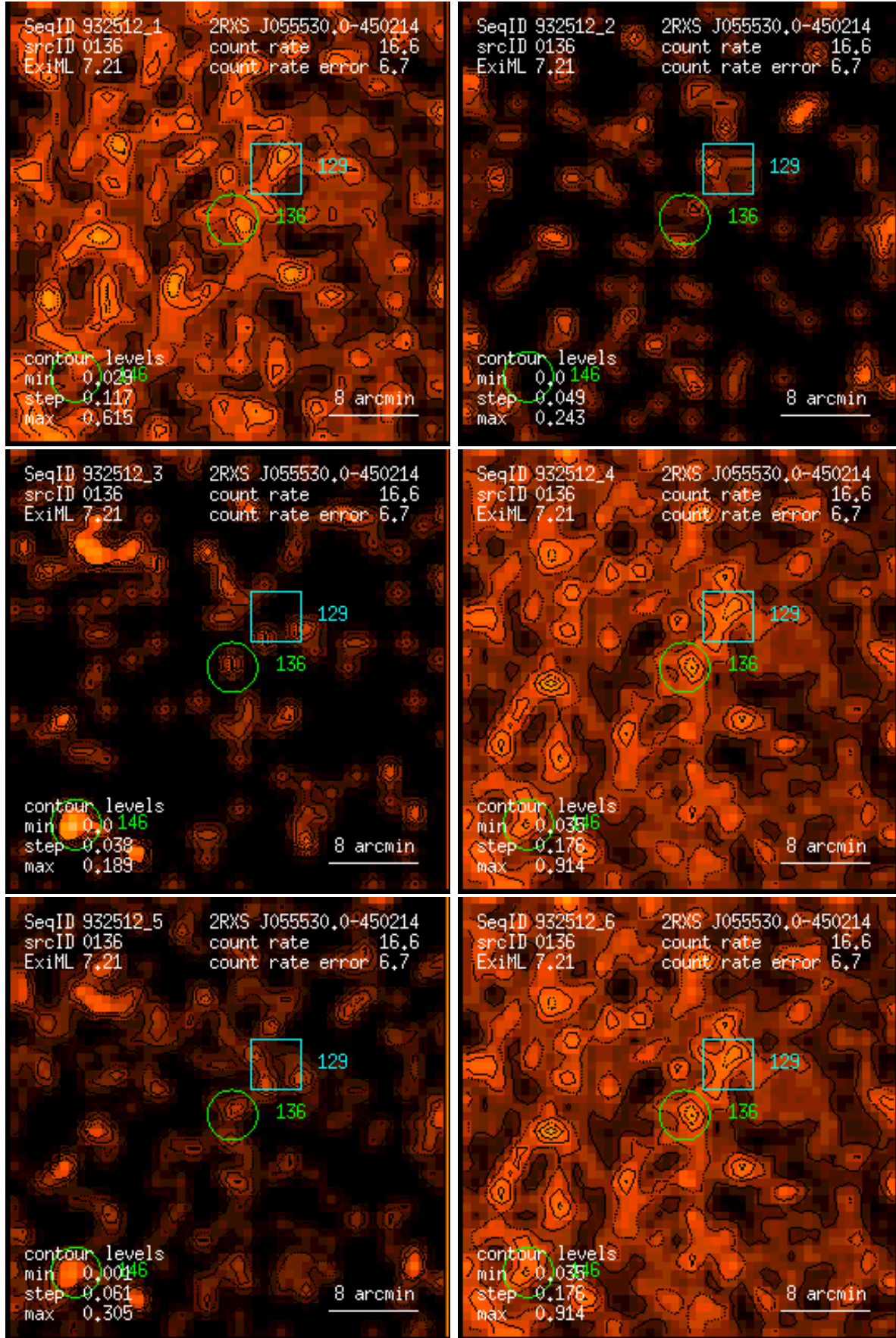
Figure 136: RASS 932512: detection 0136: band rate images, Gaussian filter: (1) PSPC channels 11 – 41, (2) 52 – 90, (3) 91 – 201, (4) 11 – 235, (5) 52 – 201, (6) 11 – 201. Broad band rates in counts/ks. Band rate contour levels in counts/ks/arcmin 2 .
