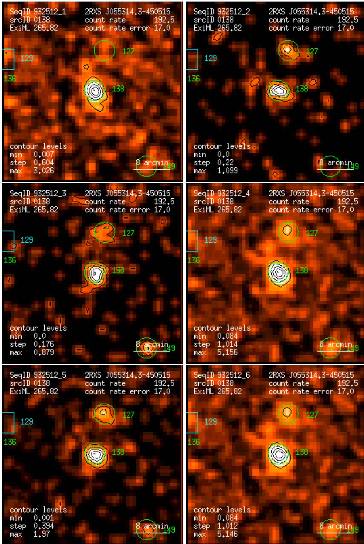
Figure 138: RASS 932512: detection 0138: band rate images, Gaussian filter: (1) PSPC channels 11 – 41, (2) 52 – 90, (3) 91 – 201, (4) 11 – 235, (5) 52 – 201, (6) 11 – 201. Broad band rates in counts/ks. Band rate contour levels in counts/ks/arcmin 2 .
